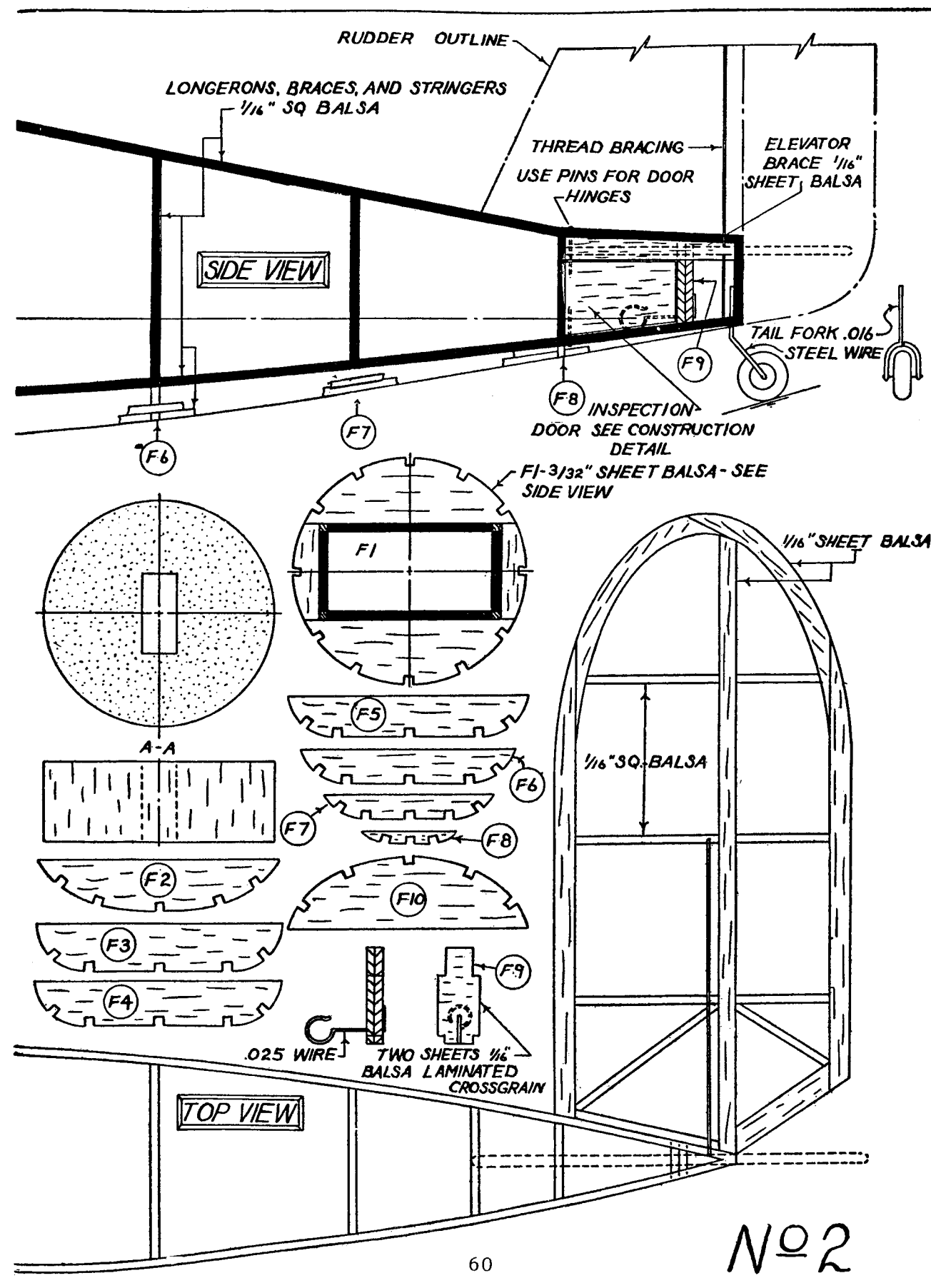
BUILD THE SENIOR PACEMAKER—Plan 2
