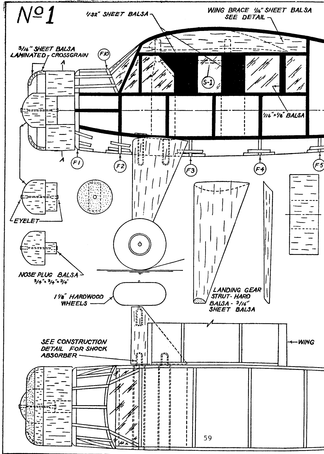
BUILD THE SENIOR PACEMAKER—Plan 1
