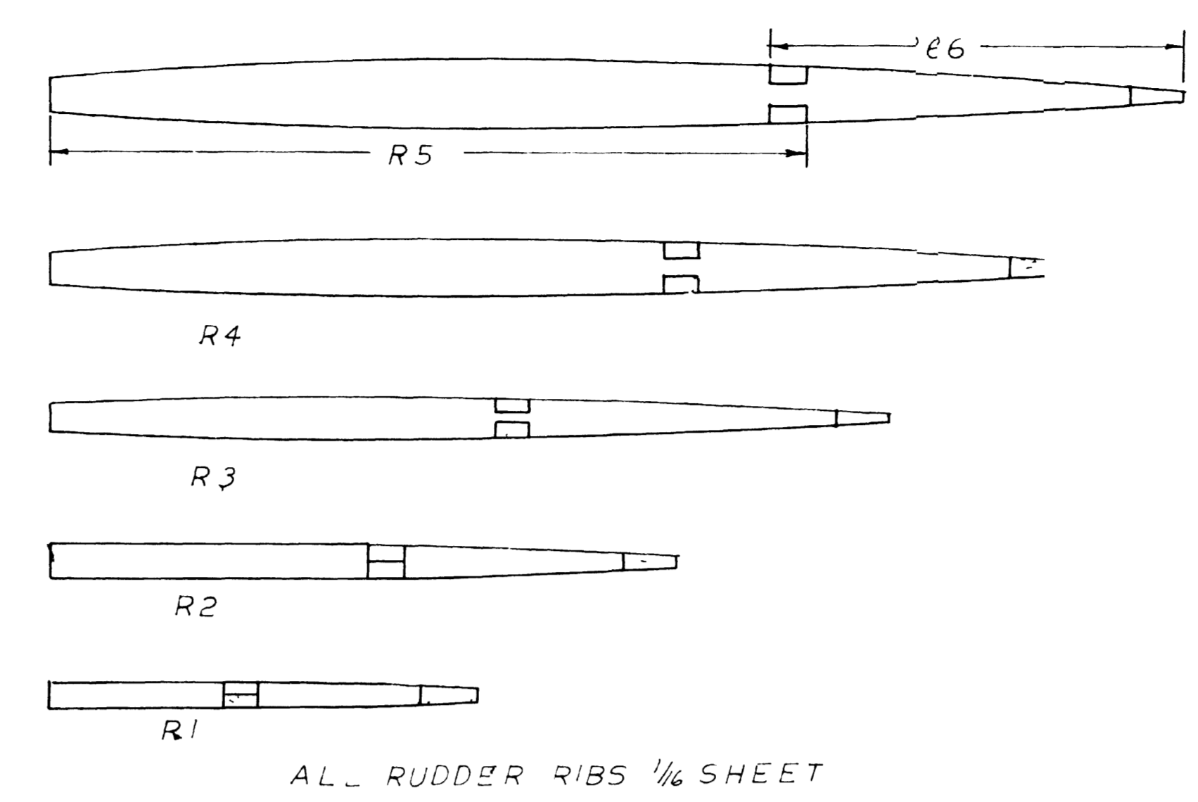
RUDDER RIBS
