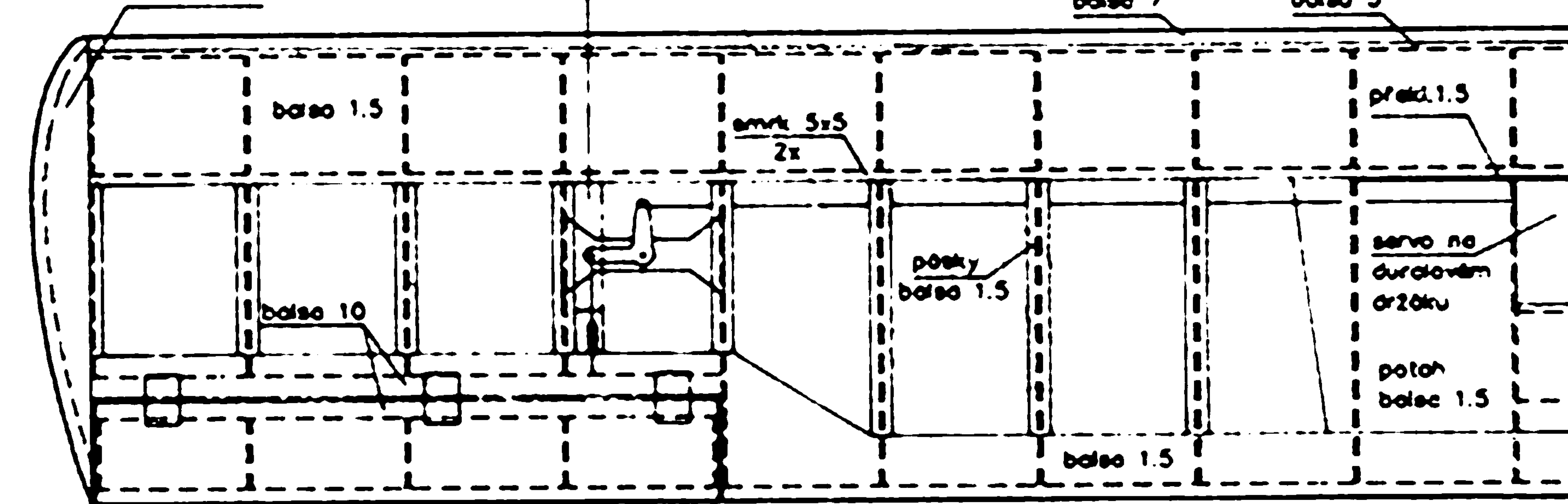
REZ B
