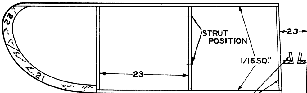
SLANT END RIBS IN WING
