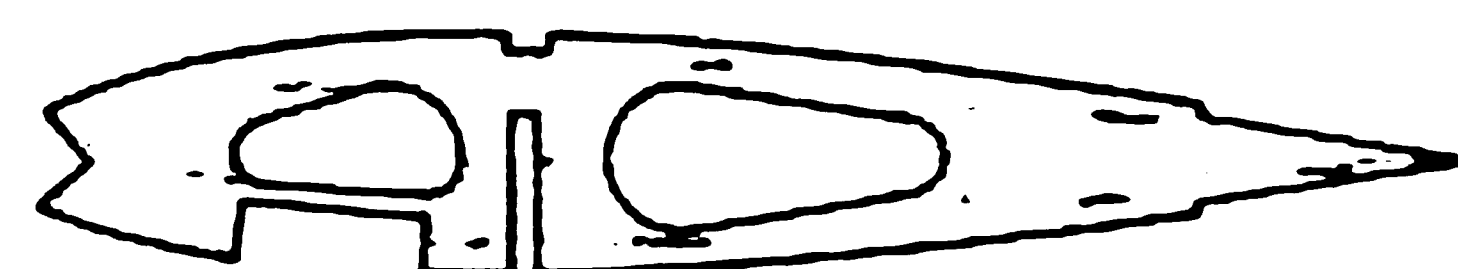
1/16" Balsa RIB, 6 REQ'D
