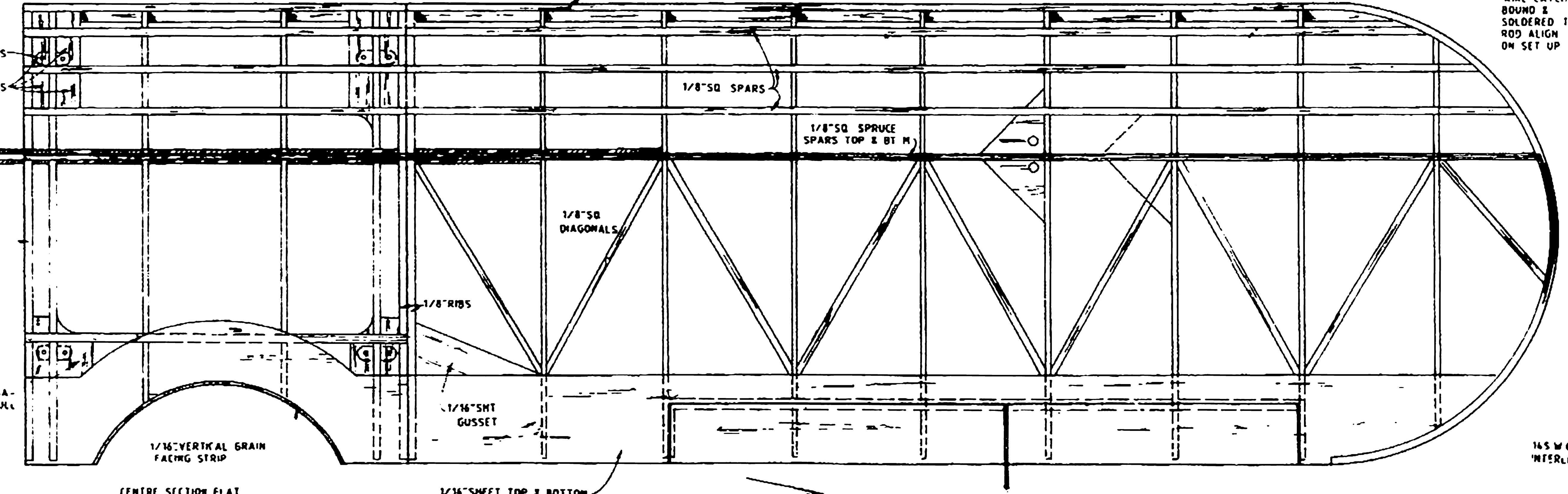
CENTRE SECTION FLAT
