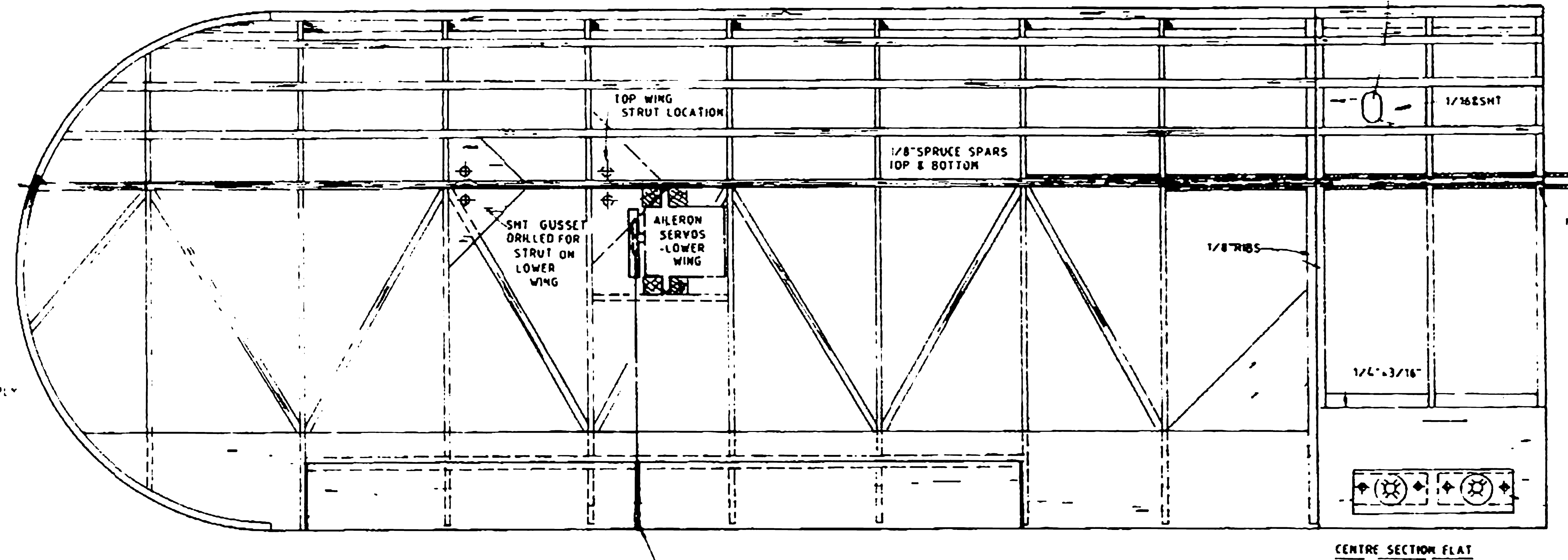
CENTRE SECTION FLAT
