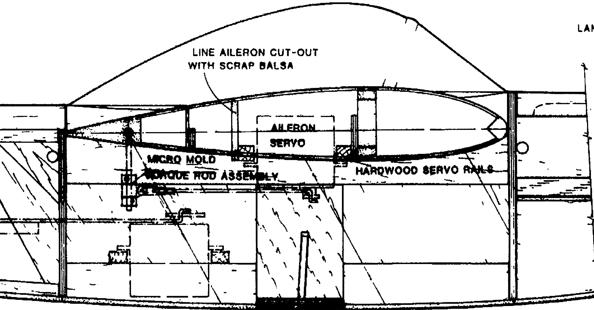
EQUIPMENT LAYOUT Aileron Version
