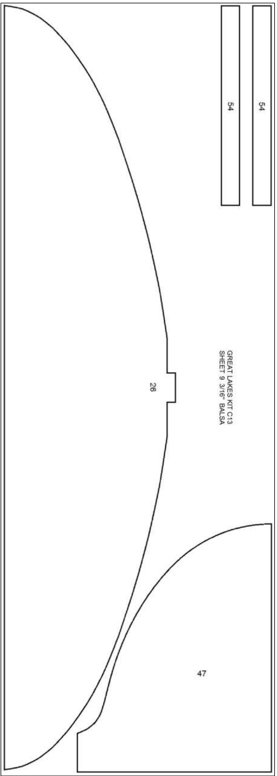
GREAT LAKES KIT C13 SHEET 8 3/32" BALSAL
