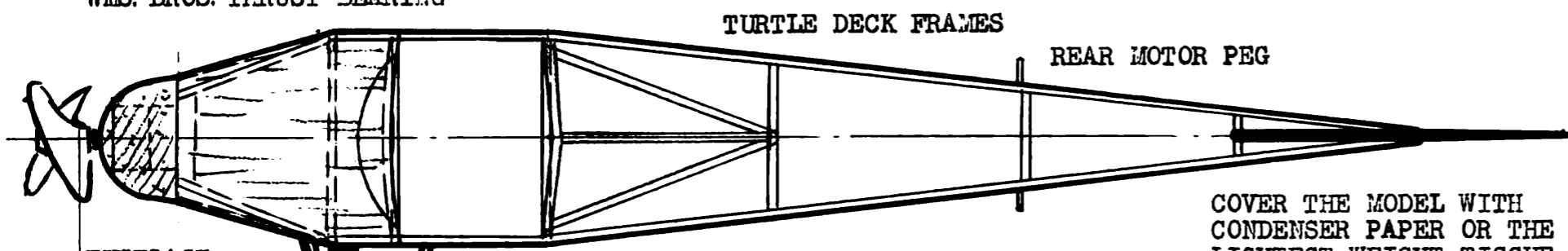
FUSELAGE TOP VIEW
