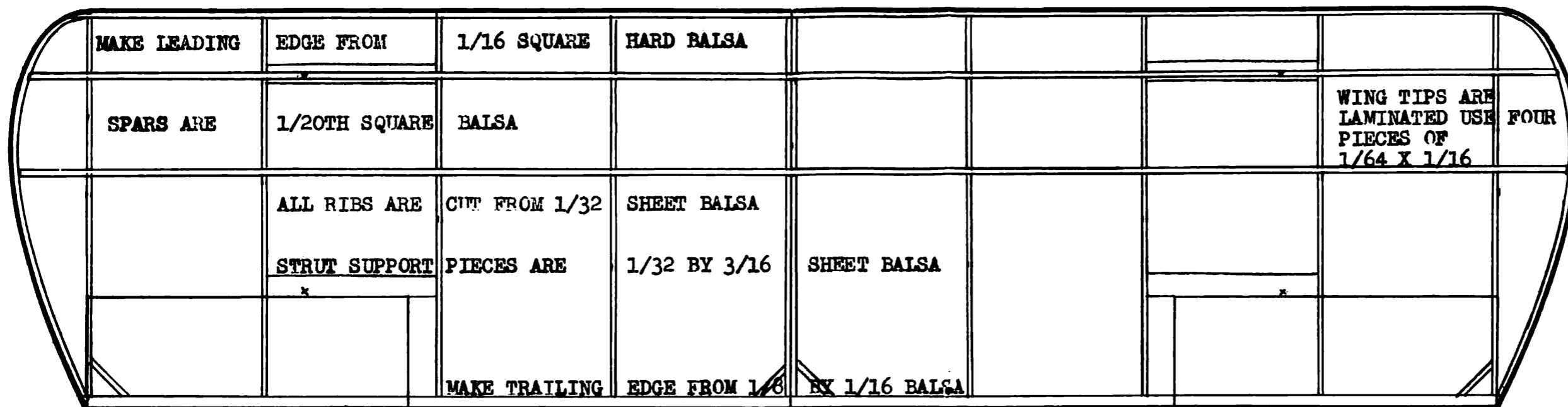
WING PLAN VIEW
