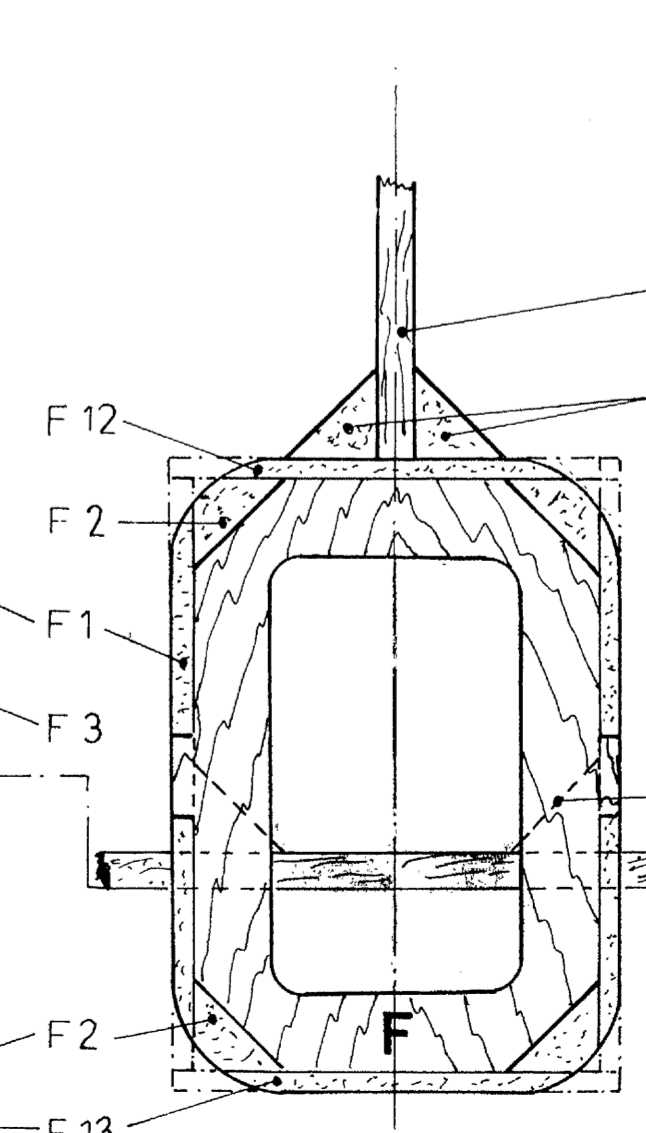
SECTION F-F
