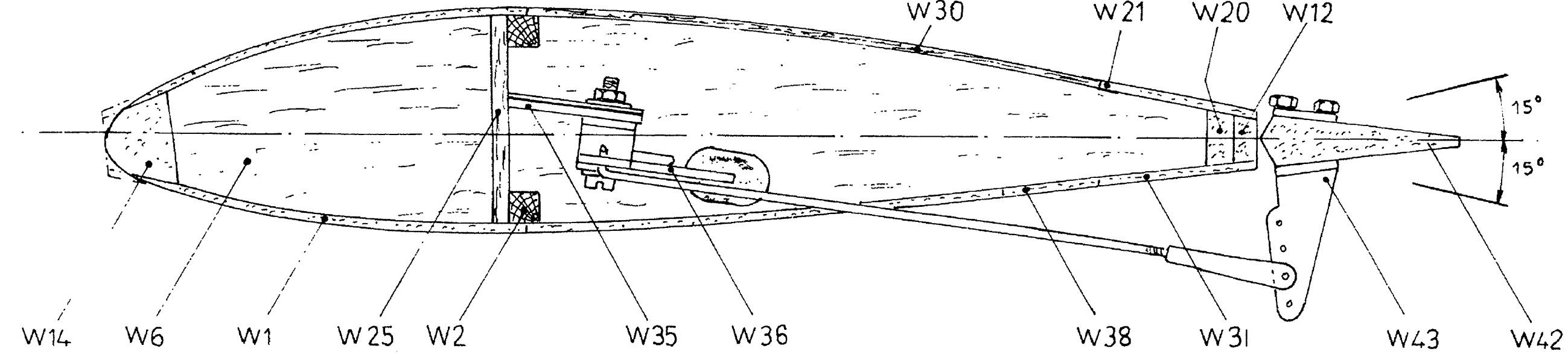
WING SECTION B-B
