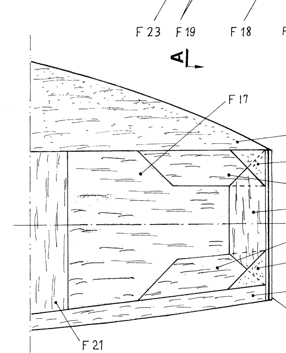
NOSE RIGHT SIDE VIEW
