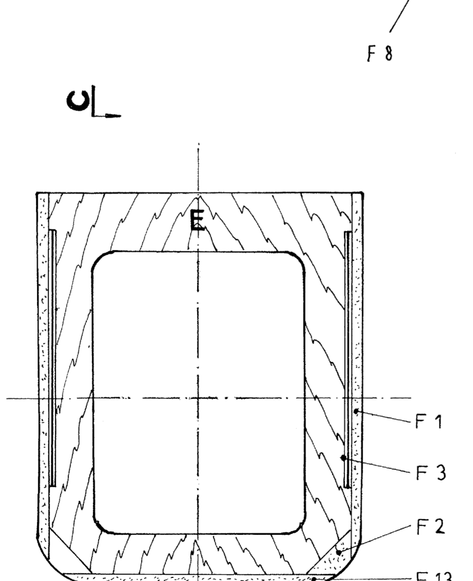
SECTION E-E
