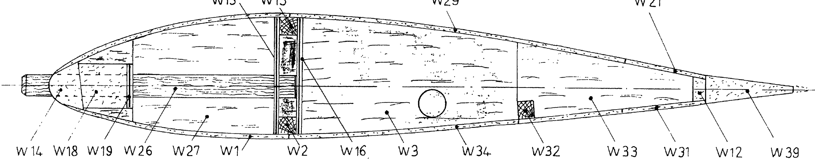
WING SECTION B-B
