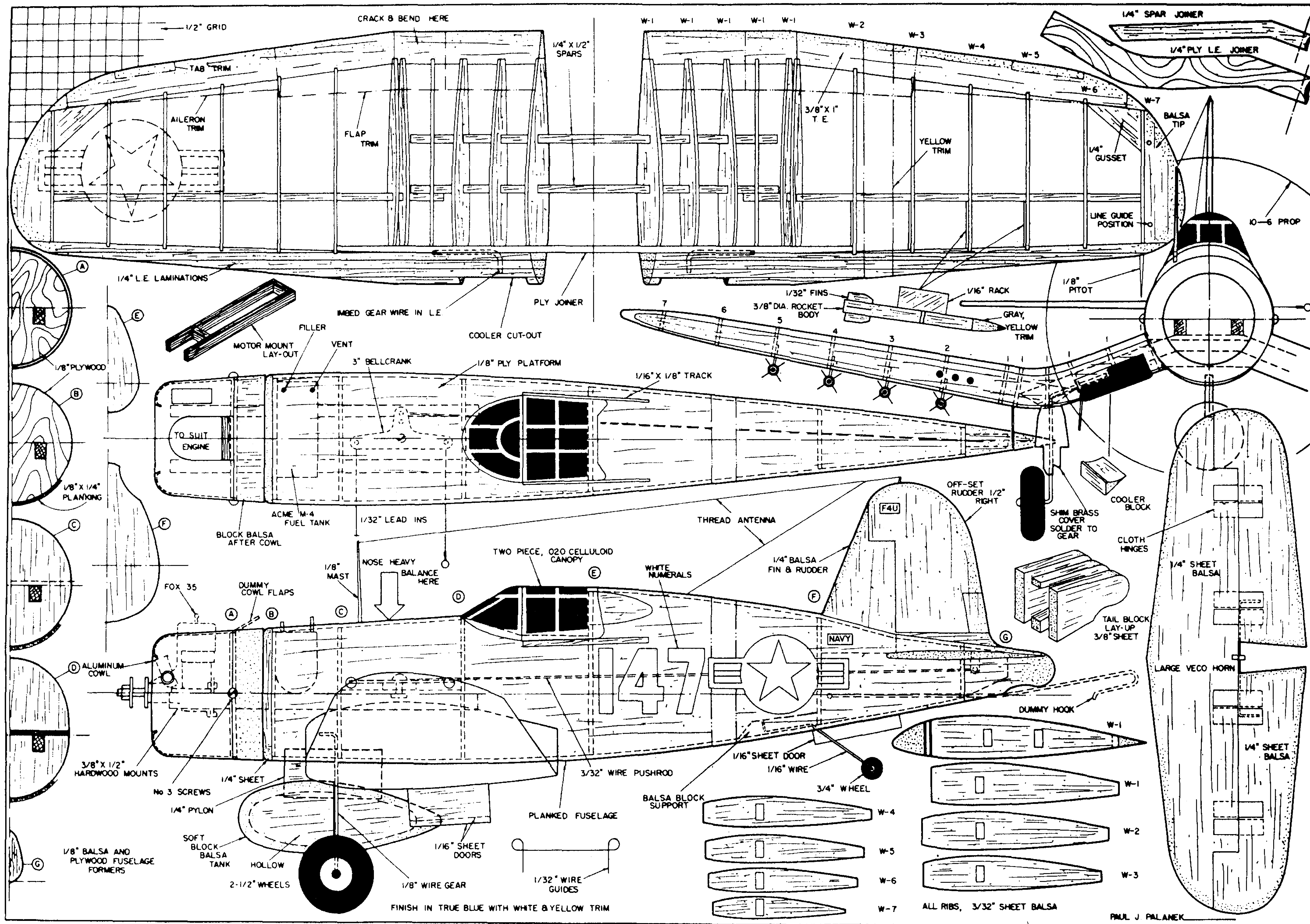
"CORSAIR" The XF4U-7 version of the famed Navy fighter by Paul Palanek. .35 engines,
