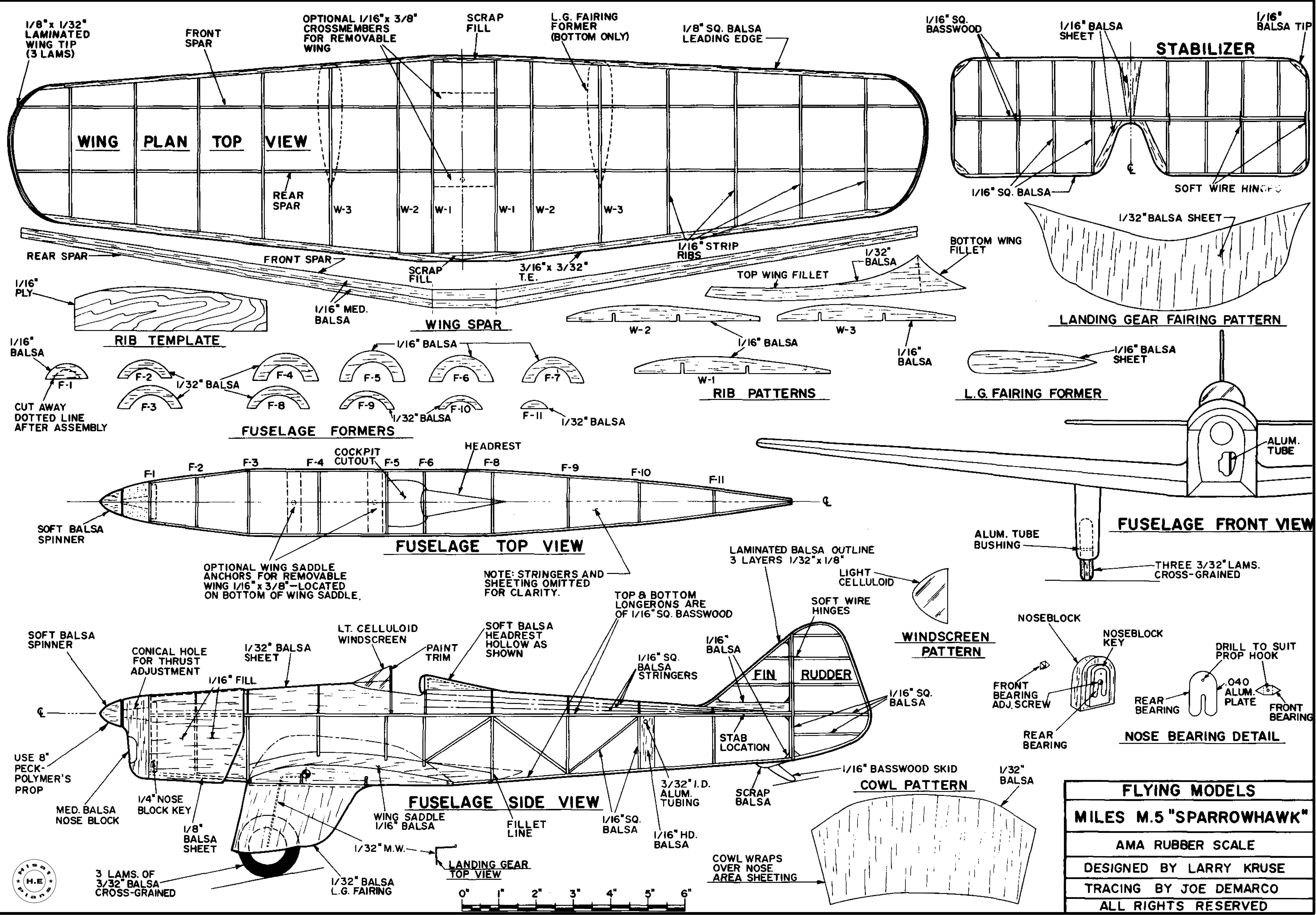
Plan CF-671
