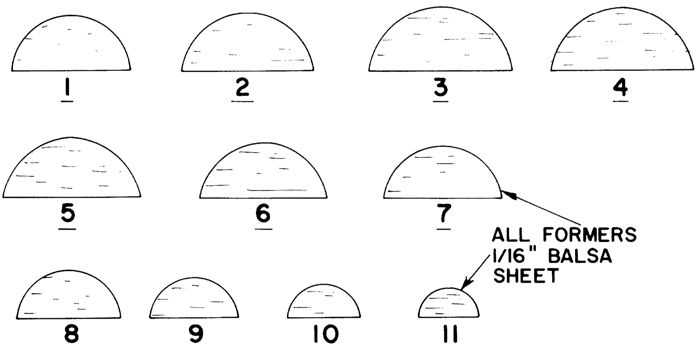
FORMER TEMPLATES
