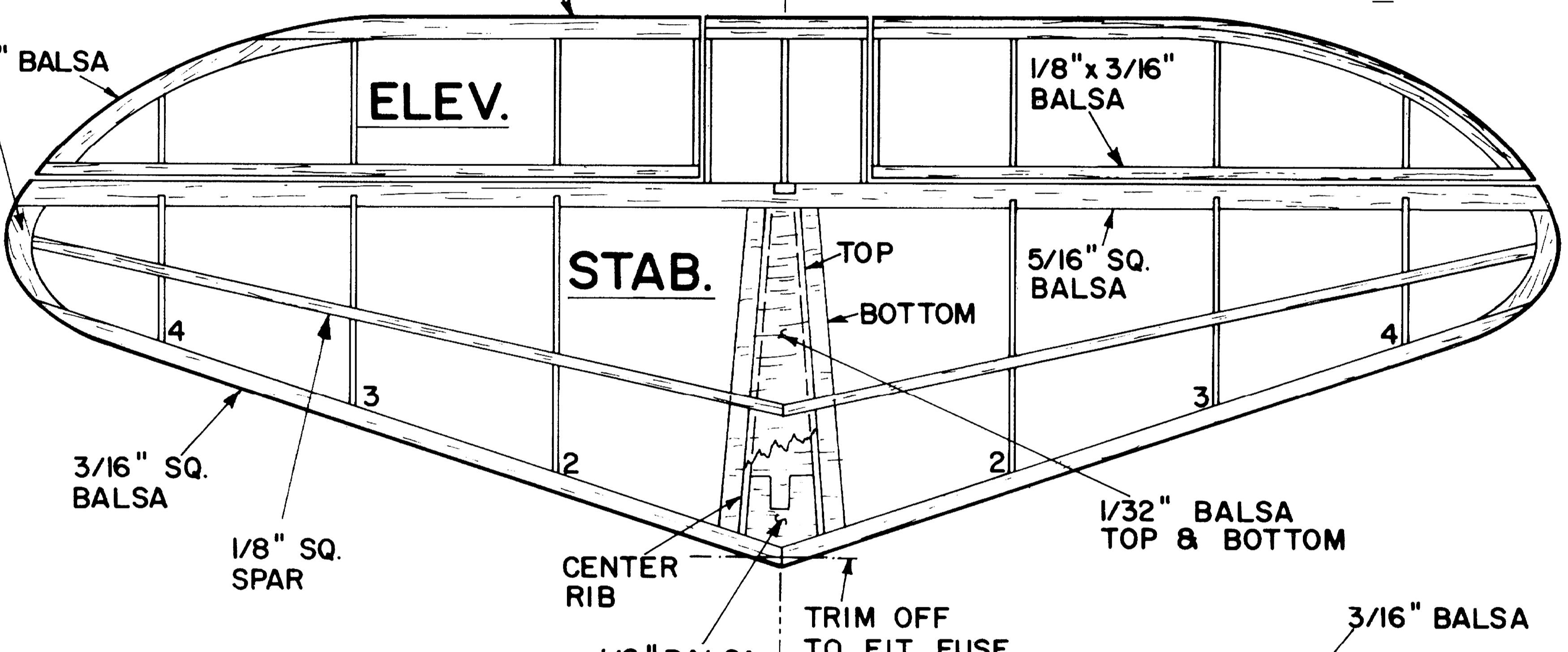
STAB. RIBS
