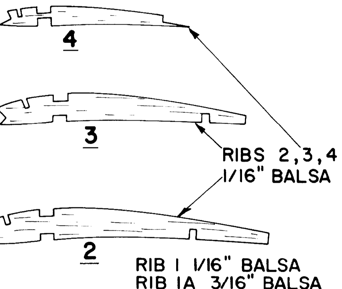
WING RIBS
