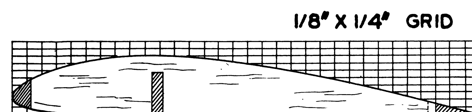
AIRFOIL MAKE RIBS FROM 3/32" BALSA
