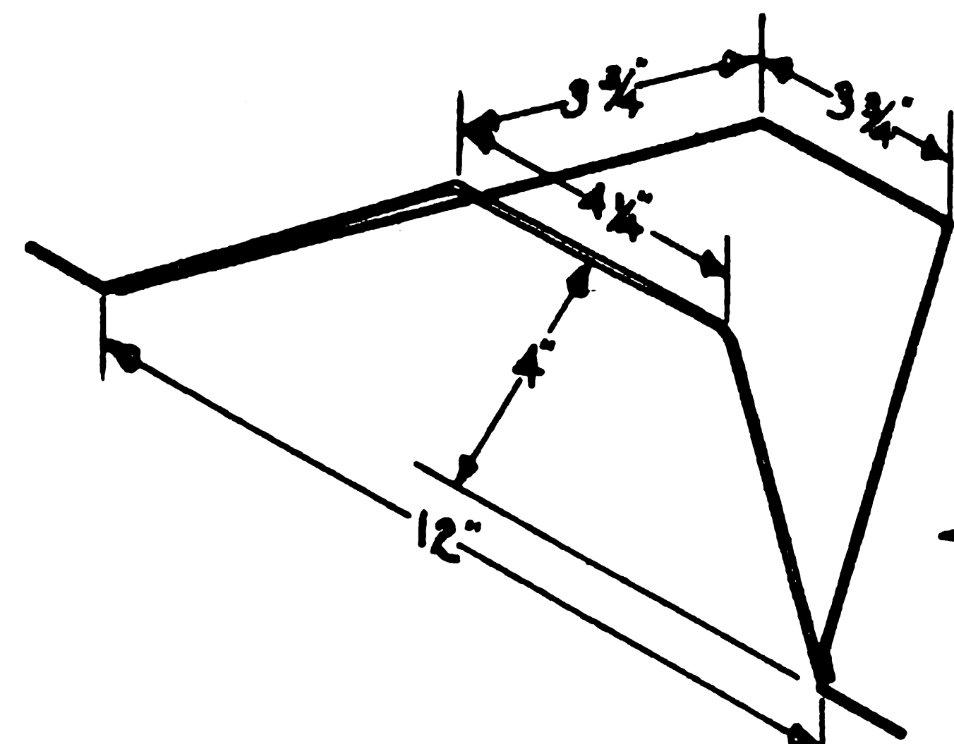
LANDING GEAR NOT TO SCALE
