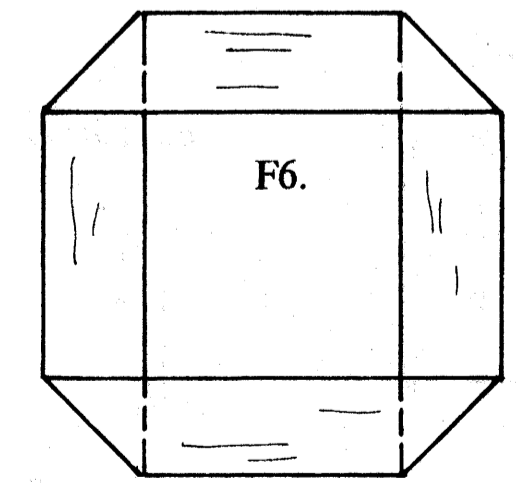
Make up formers F2,F3,F6&F7 from 1/2" x 1/4" balsa.
