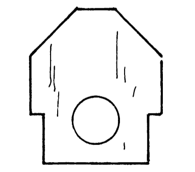
F8 from 3/16" balsa.
