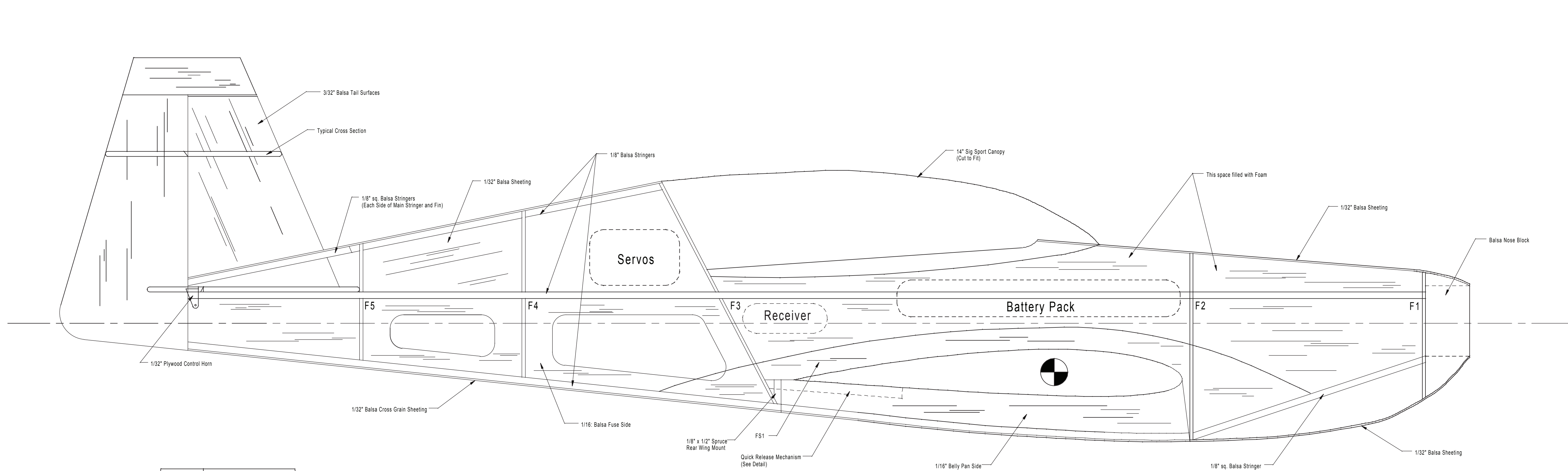
Fuselage Side View
