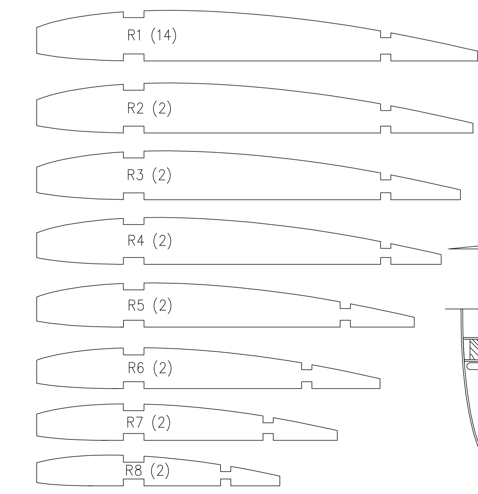
RIBS
