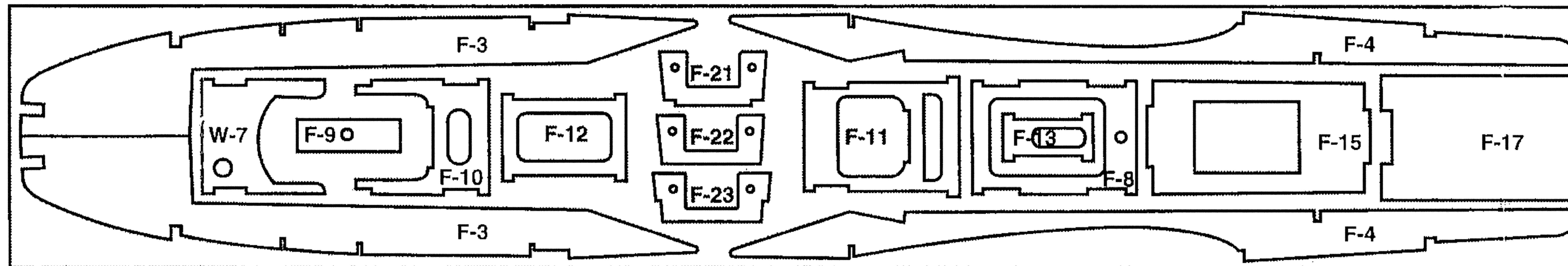
COMBO Fuse 25S
