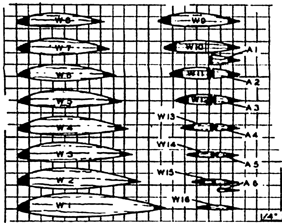
WING SECTIONS - 1 EACH 1/16" SHEET
