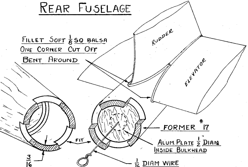
Below: Because of the tensioner, the rear fuselage section stays attached without hooks, etc.
