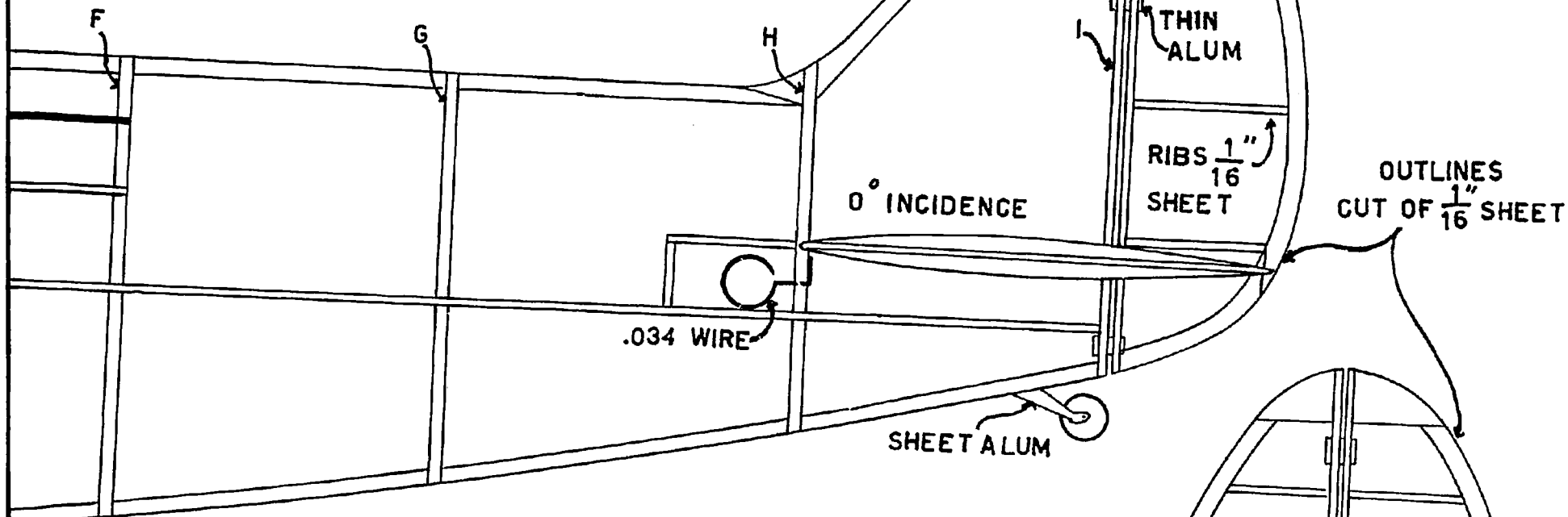
TYPICAL TAIL SECTION
