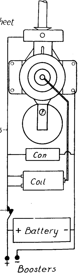
Wiring diagram
