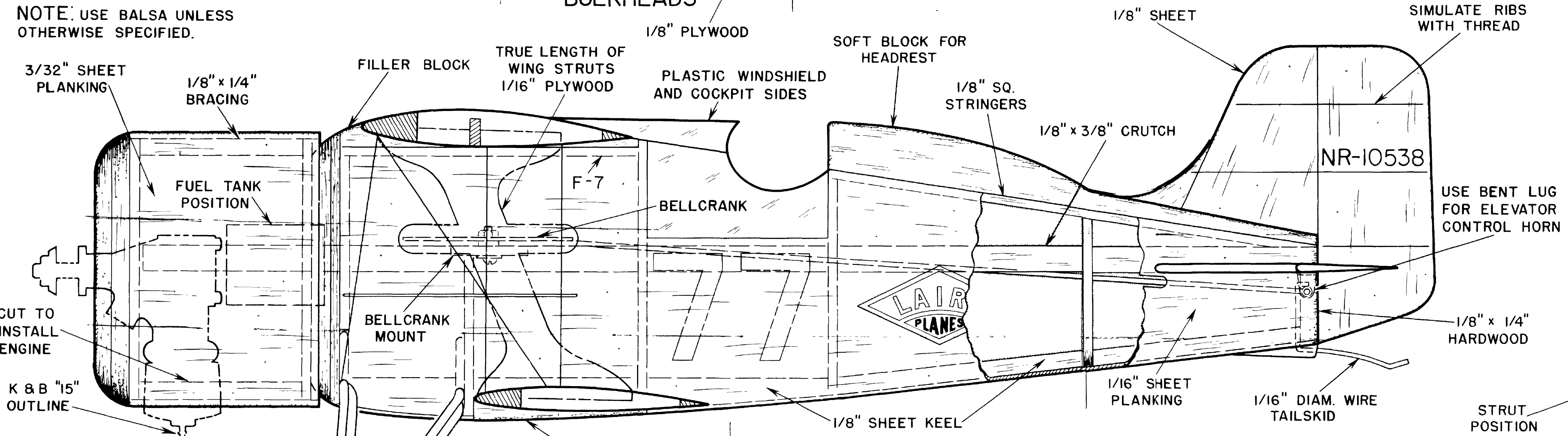
FUSELAGE SIDE VIEW
