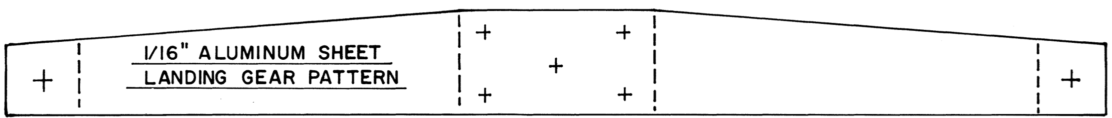
LANDING GEAR FRONT VIEW
