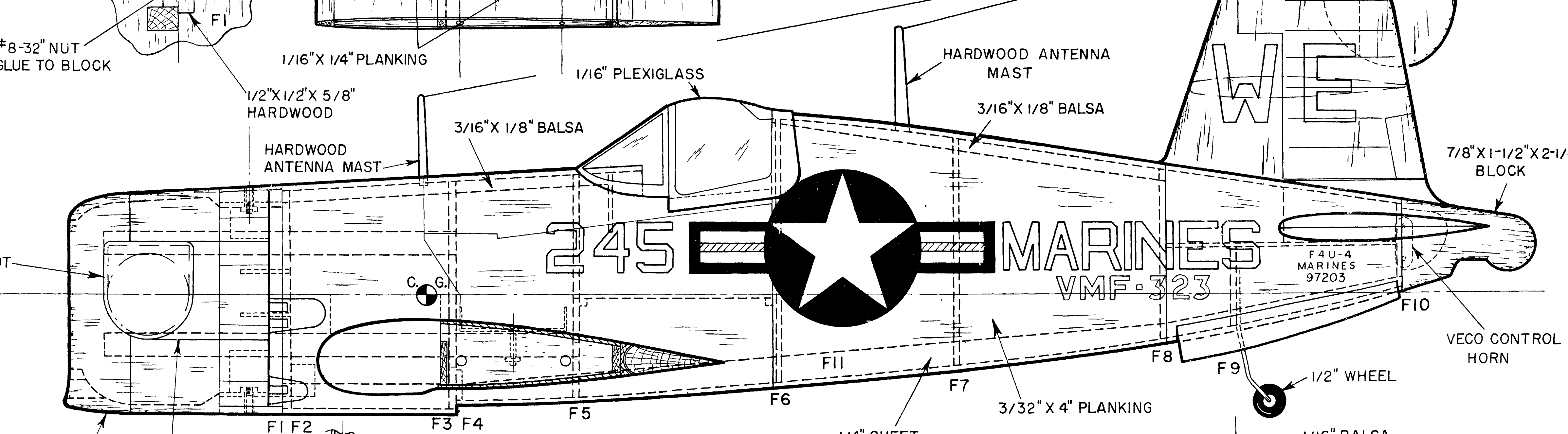
FUSELAGE SIDE VIEW
