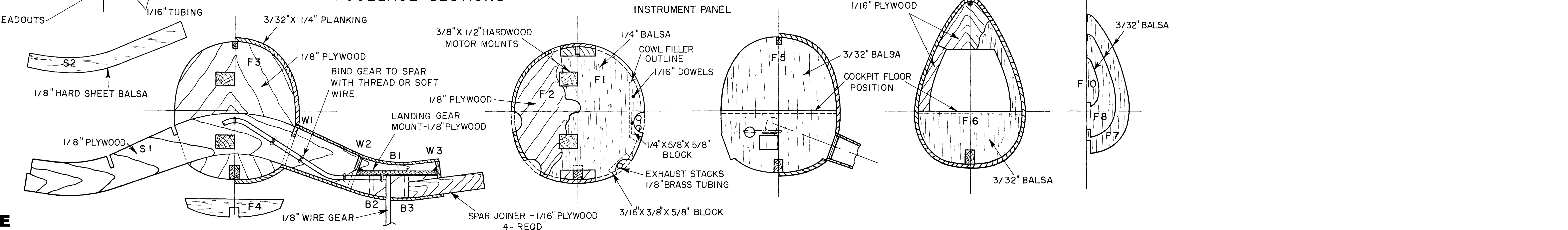
FUSELAGE SECTIONS
