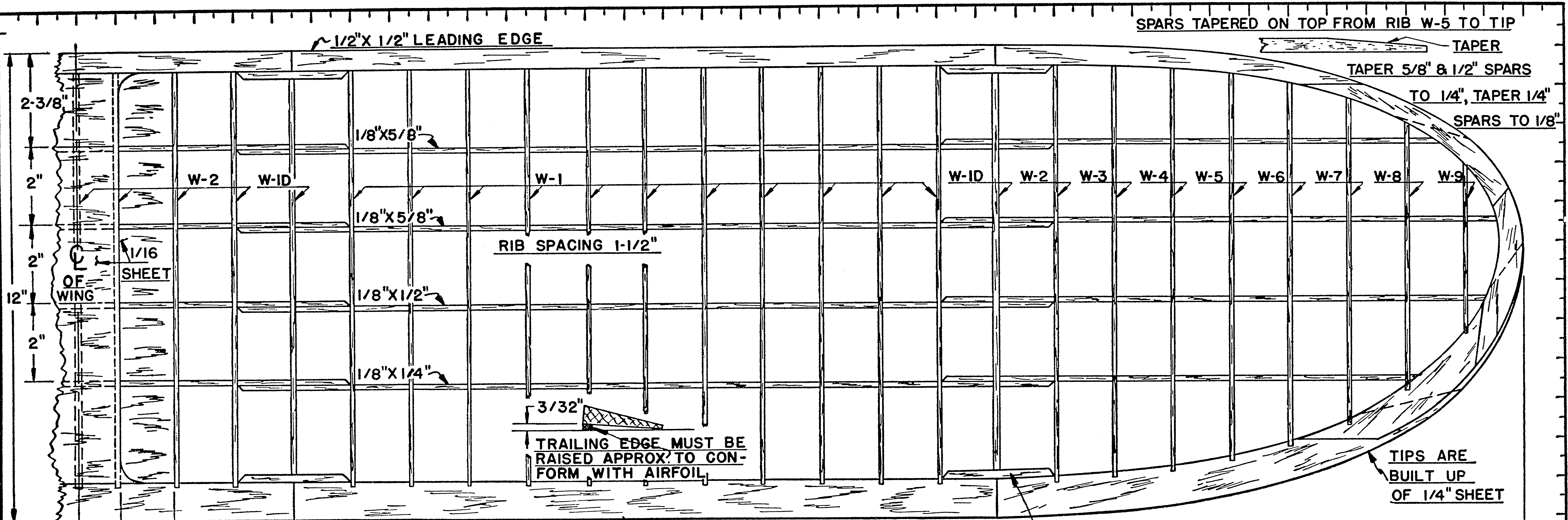
WING LAYOUT
