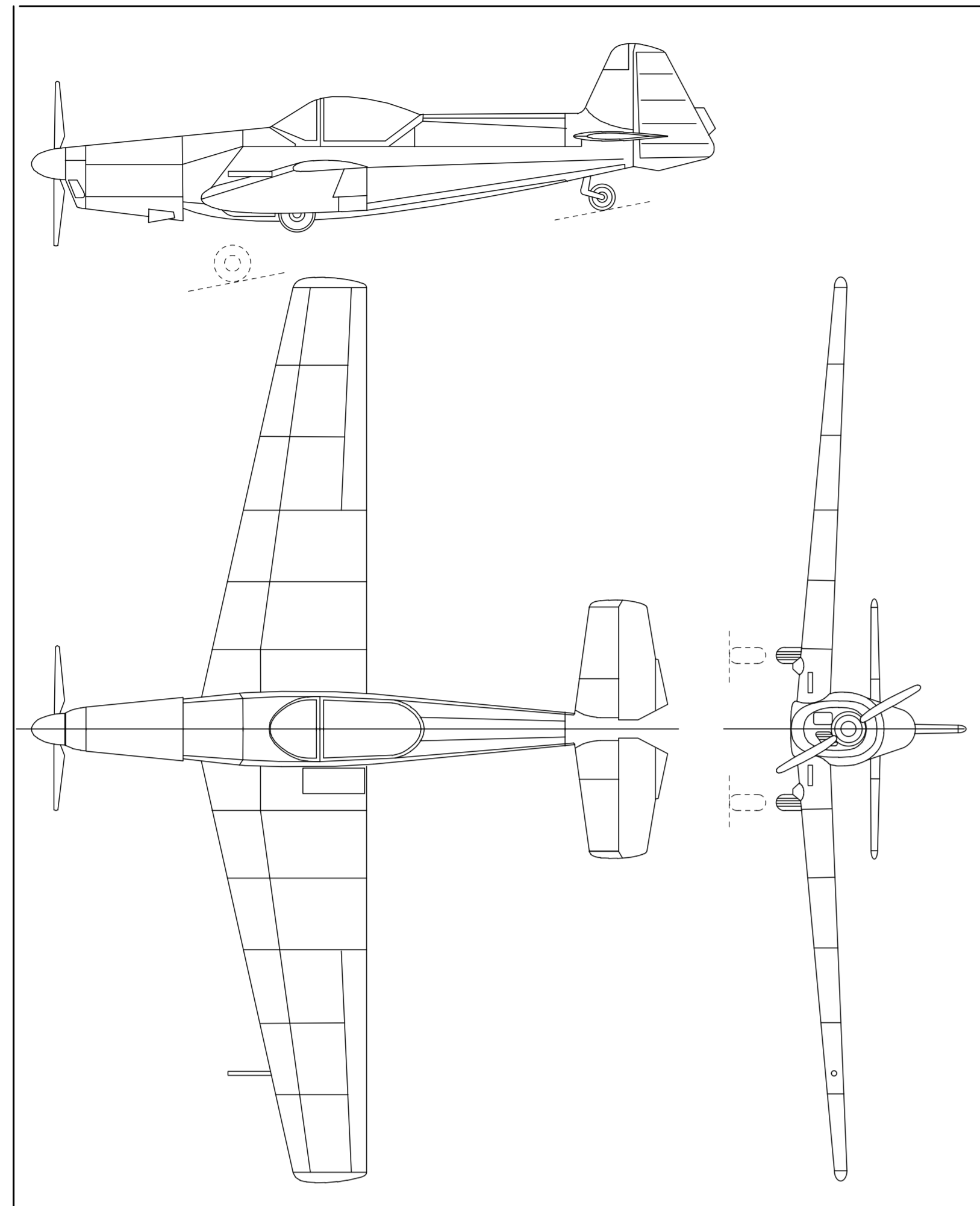
TRITTICO ZLIN 526 AS Full-size - Scala 1:50
