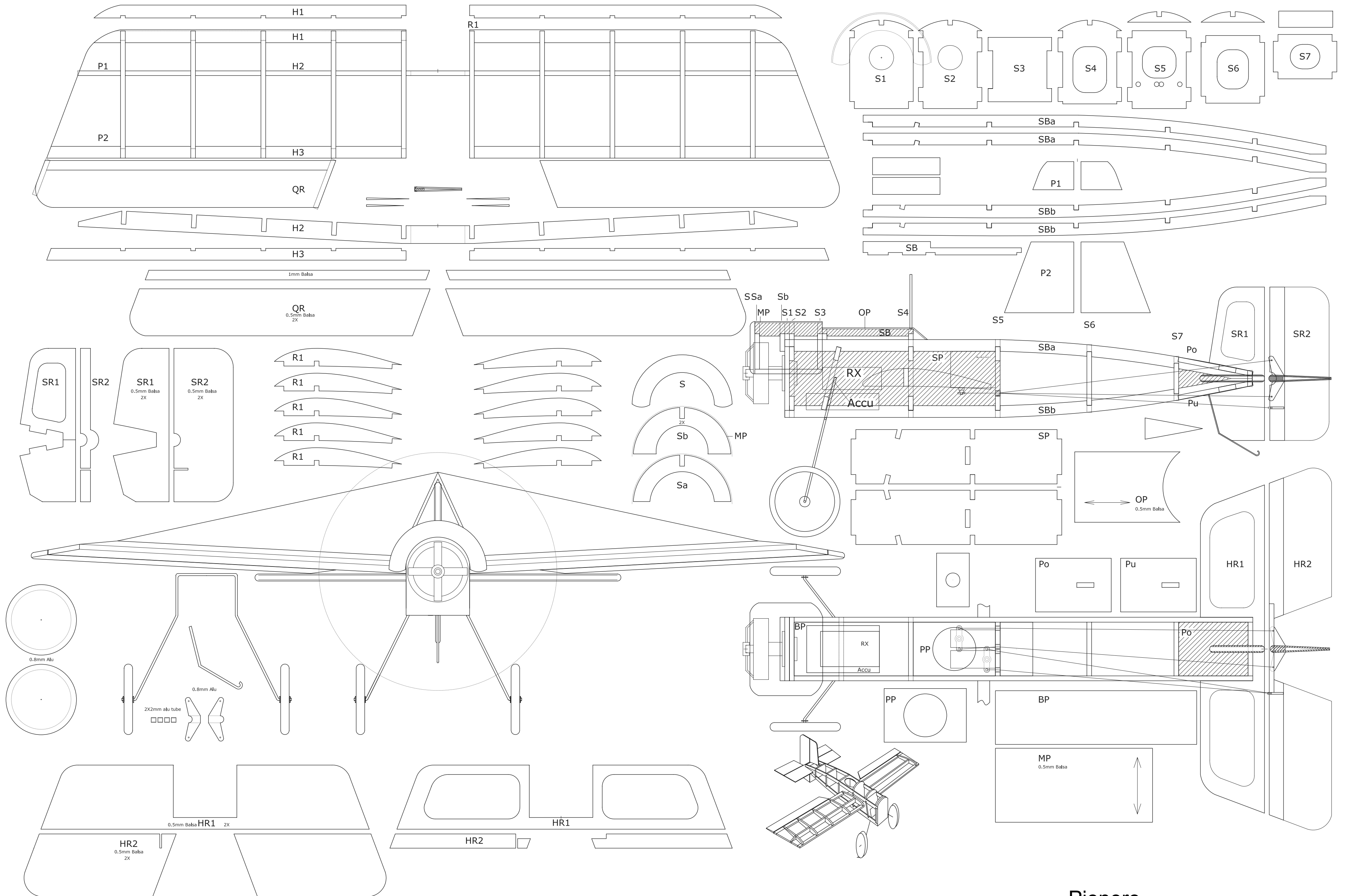
Pionero Peanut Scale by Arno Diemer All Wood is 2mm Balsa Wood unless stated otherwise
