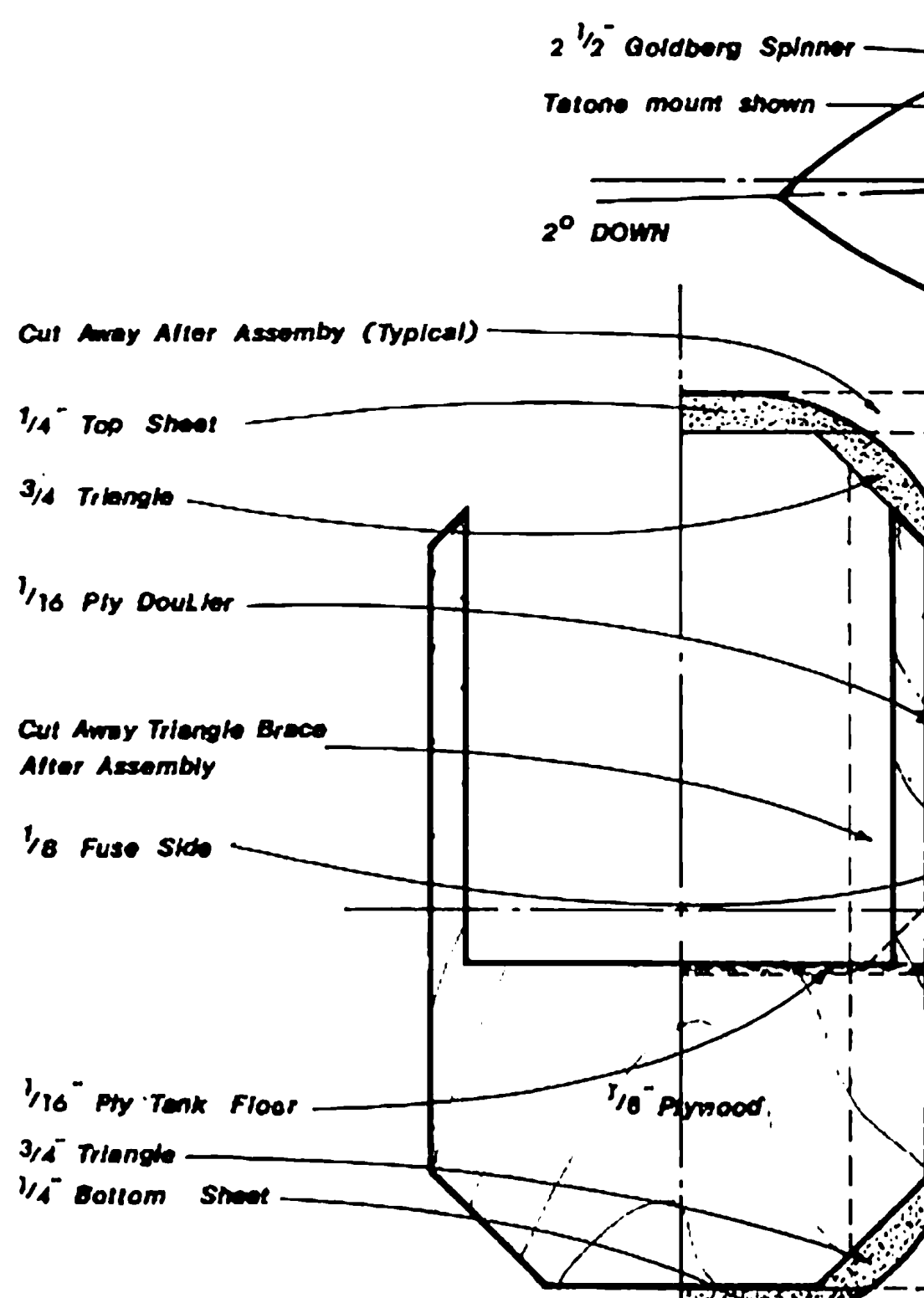
Forward Bulkhead F2
