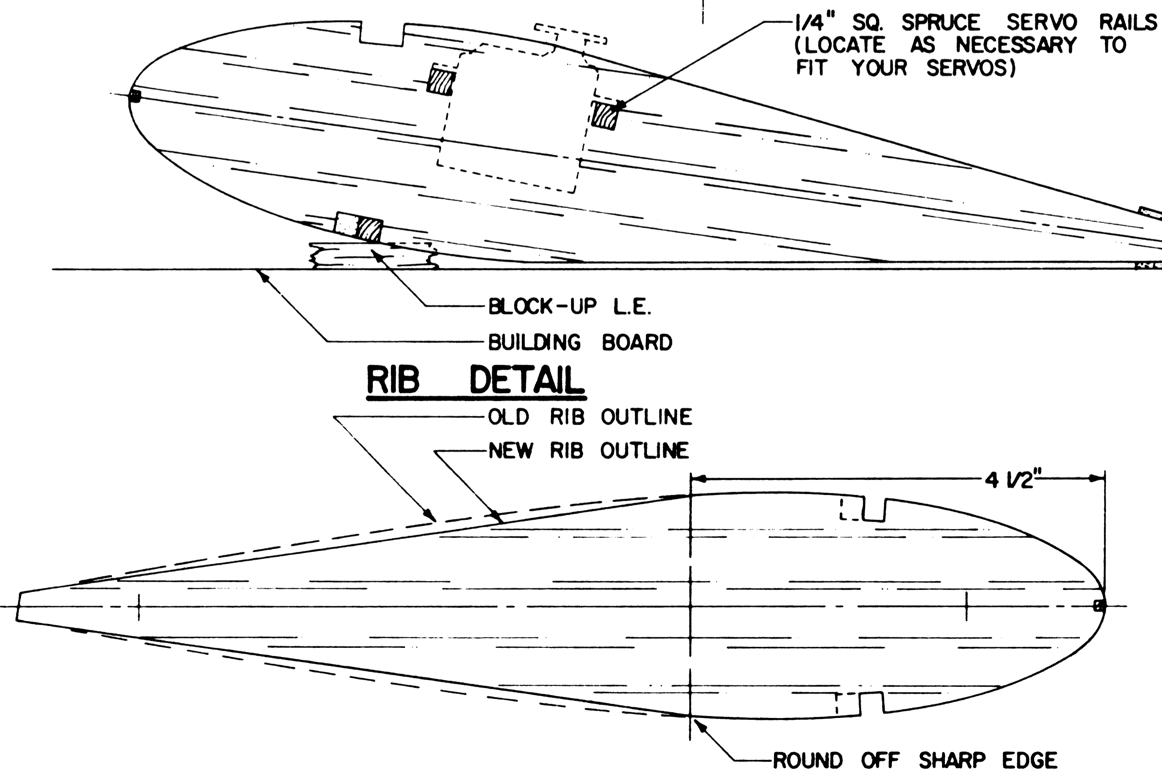
WING PLAN
