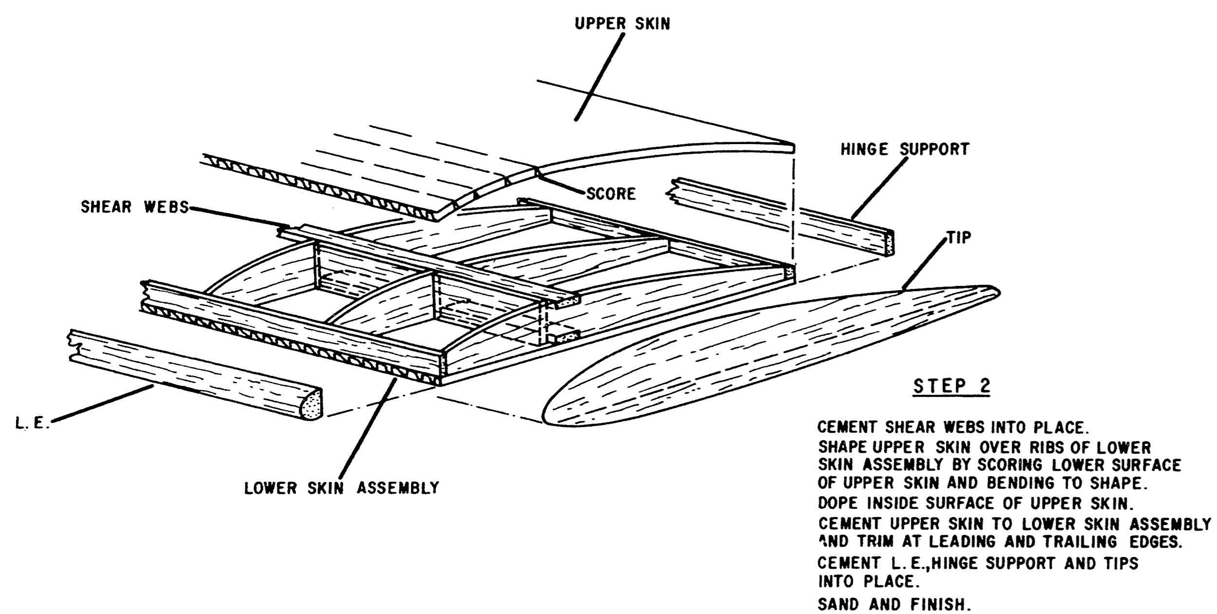
WING CONSTRUCTION- FINAL ASSEMBLY FIGURE 7
