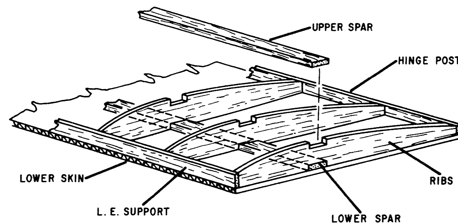
RUDDER CONSTRUCTION FIGURE 2
