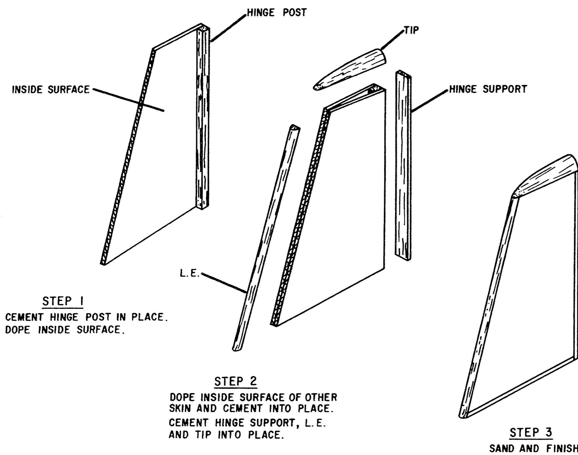
VERTICAL STABILIZER CONSTRUCTION FIGURE 1
