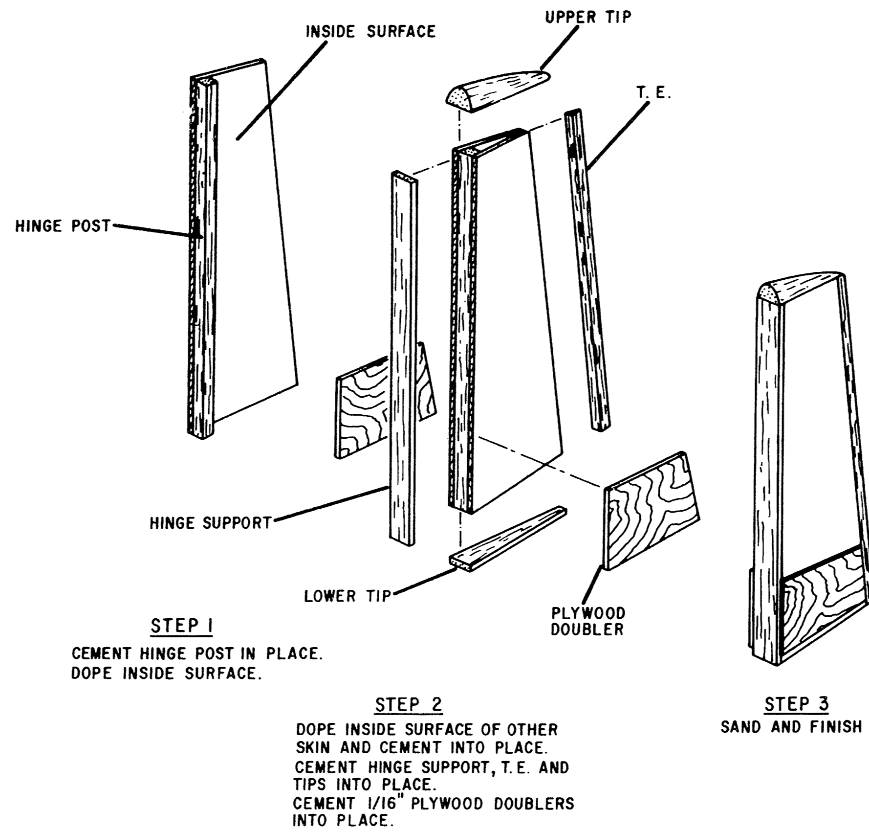
RUDDER CONSTRUCTION FIGURE 2
