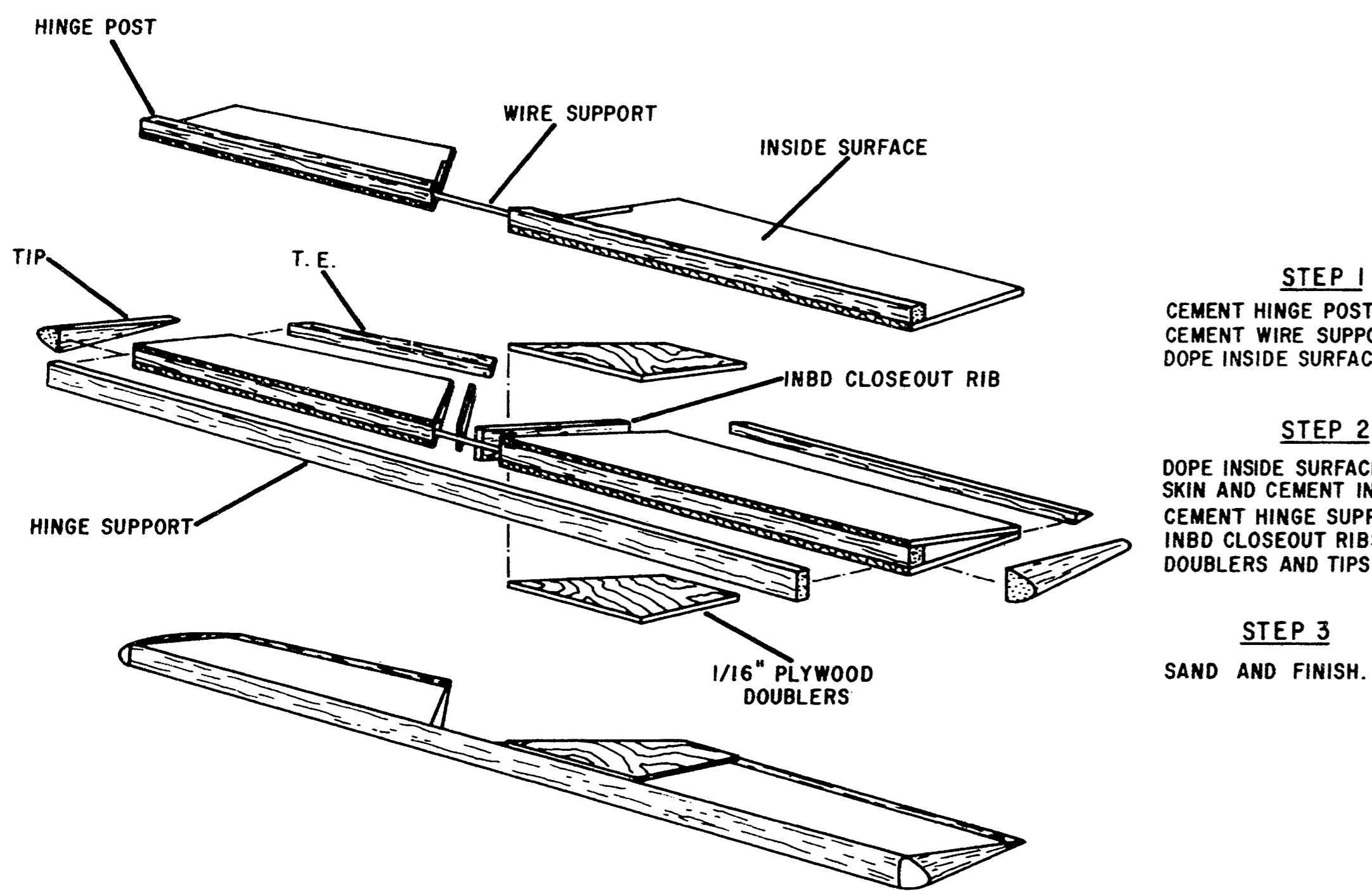
VERTICAL STABILIZER CONSTRUCTION FIGURE 1
