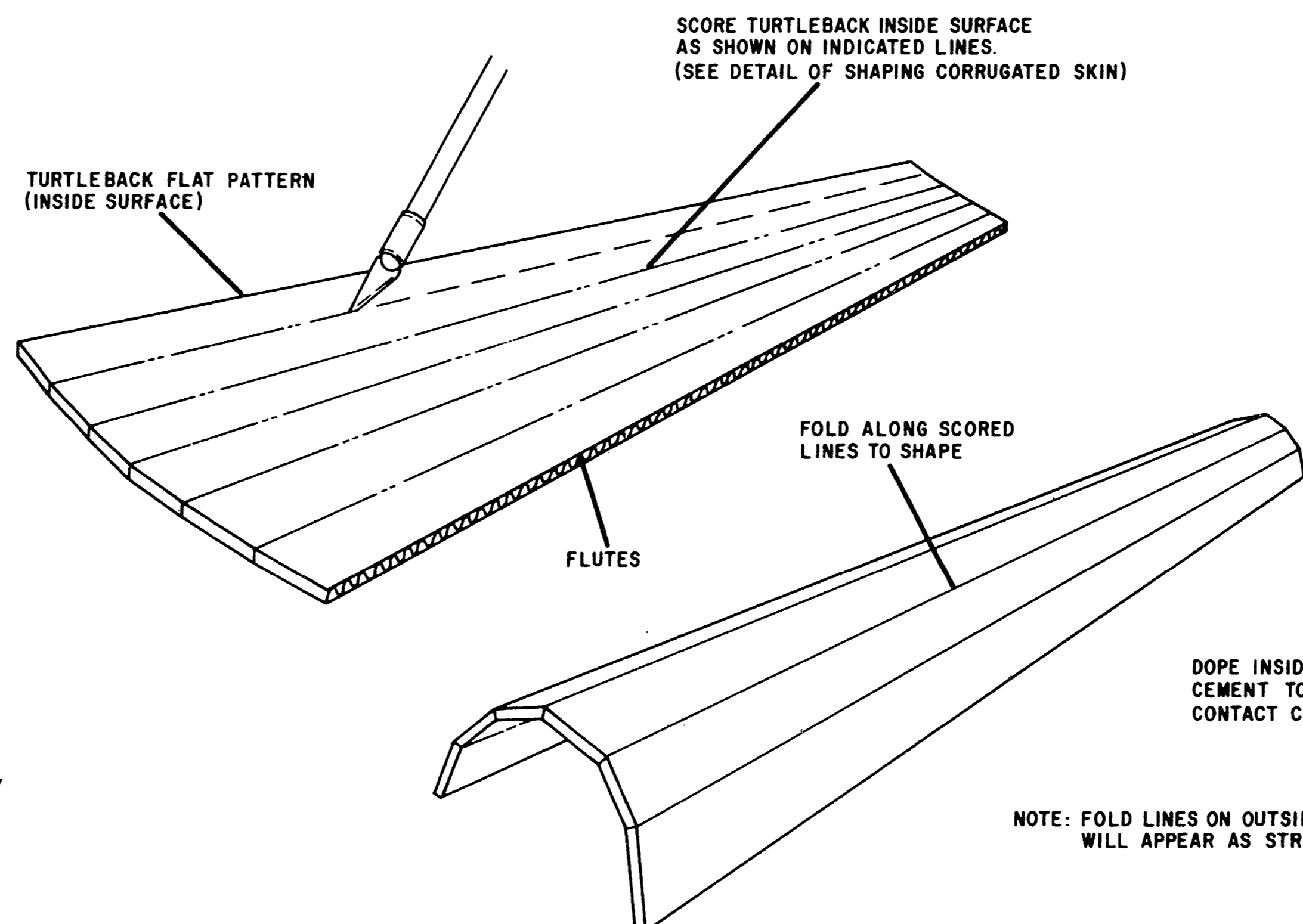
TURTLEBACK CONSTRUCTION FIGURE 8
