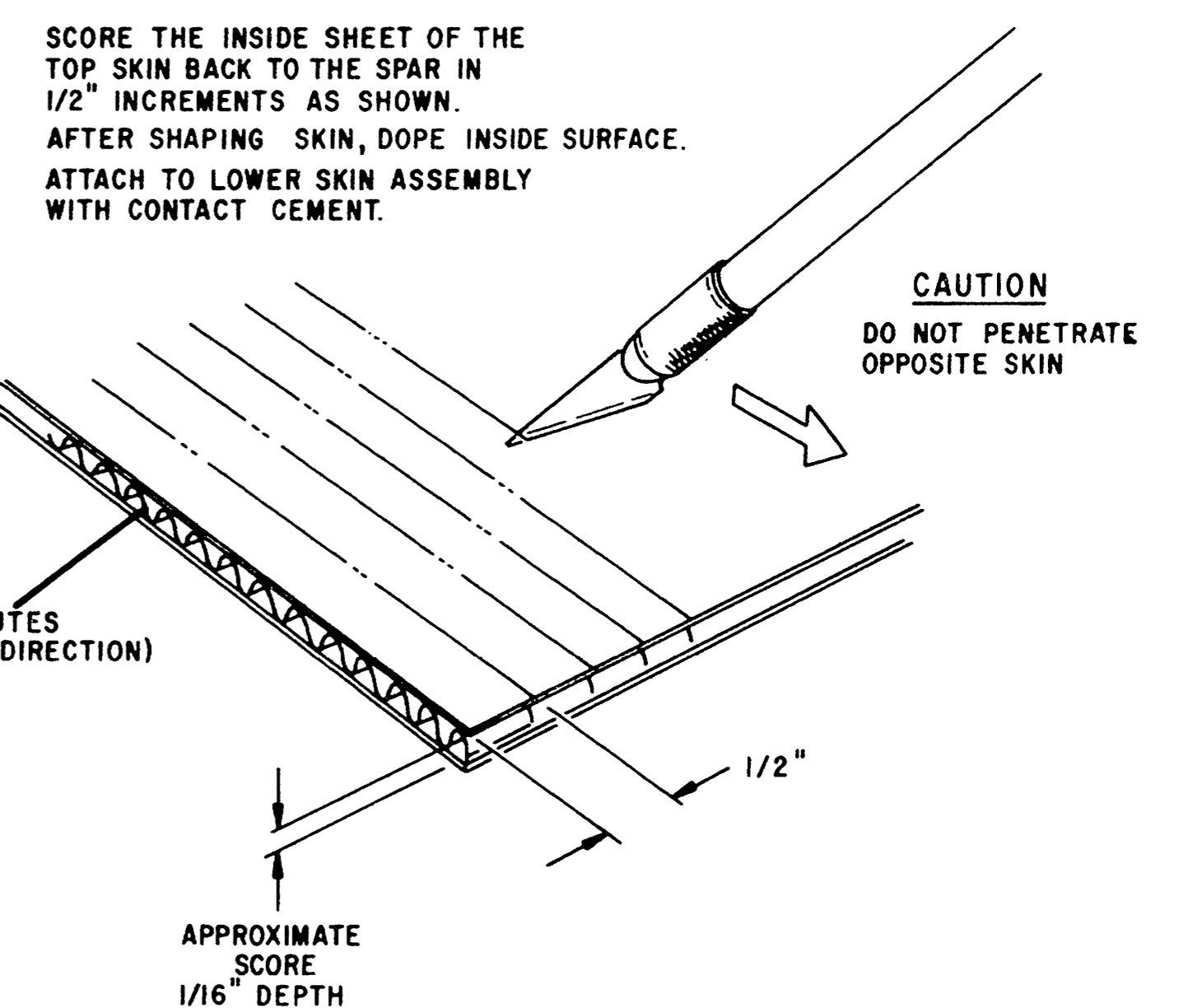
SHAPING CORRUGATED SKIN FIGURE 6
