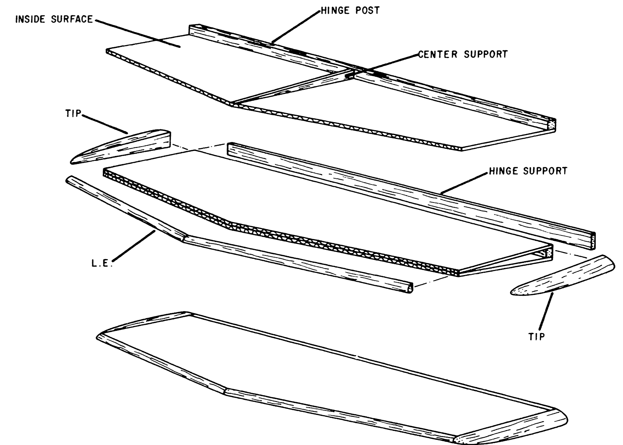
HORIZONTAL STABILIZER CONSTRUCTION FIGURE 3
