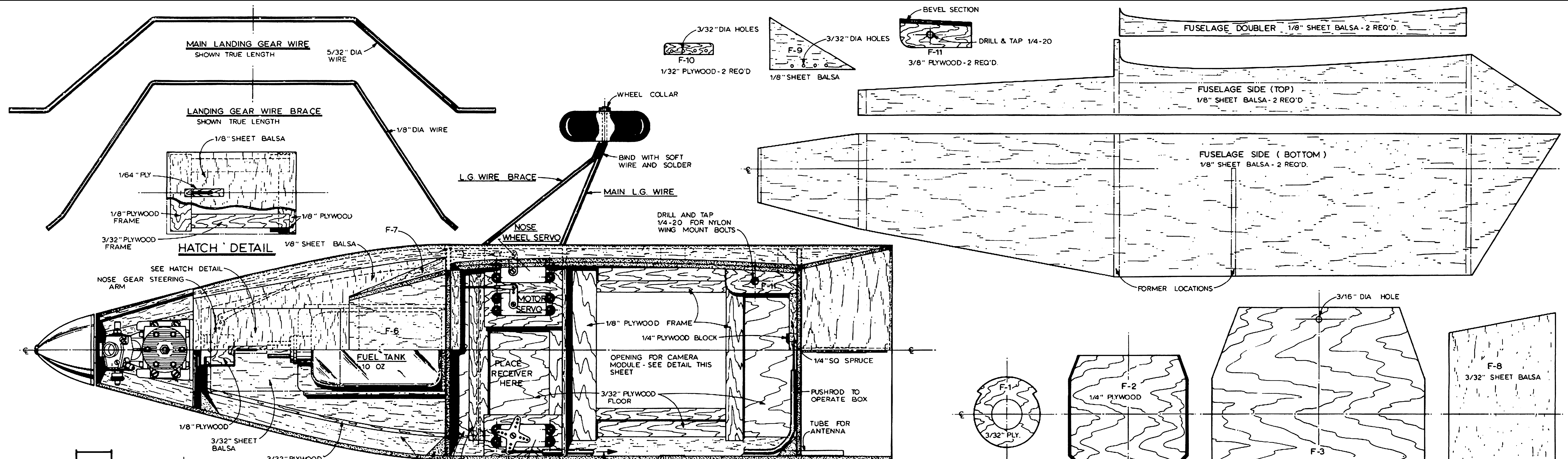
FUSELAGE PLAN VIEW
