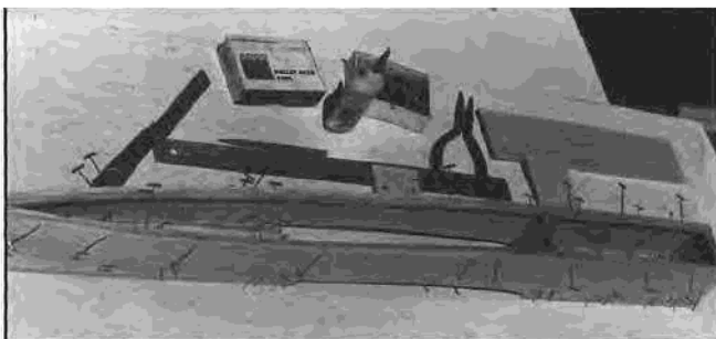
After fuselage sides are joined and CA'd at rear, pin top 1/4" sq. longerons in place and CA them.
