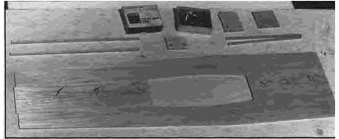
Lay 1/4" fuselage top and front balsa pieces down on building surface, line them up using fuselage sides, mark pencil line on center of the top front and rear pieces, pin them in place.
