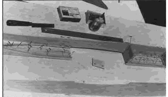
Pin and CA fuselage side in place on fuselage top front and the first 2" of fuselage rear top. Do the same for other side, then join at rear.
