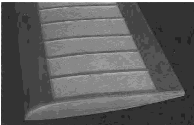
After sheeting bottom of wing panel, sand leading edge undercap flush with sheeting. Cement and trim the 3/8" leading edge cap to shape shown on plans. Note steep top on leading edge and fairly flat bottom. Glue the 1/4" balsa tips in place and sand to shape.
