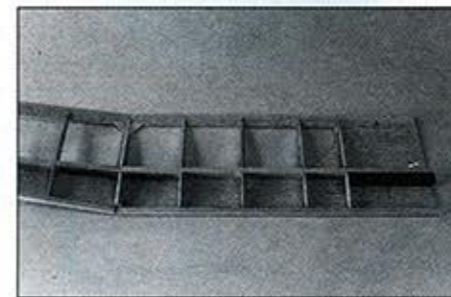
Polyhedral joint and wing rod support. Note the root rib and the first inner board ribs and root are glued in.
