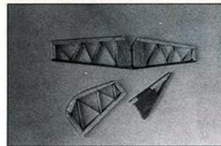
Rudder, vertical stabilizer, stabilator assemblies.
