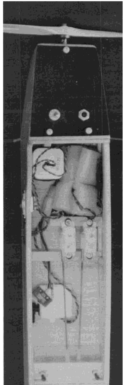
BELOW & RIGHT: The VW has an ingenious radio and battery installation. The bottom compartment houses flight battery, the top one houses the receiver, servos, RX pack.
