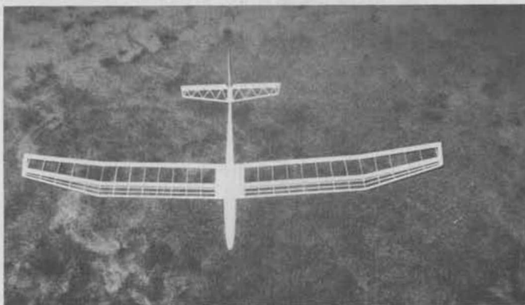
Here's the Tossette, bare naked and awaiting covering. The author chose to cover his with Super MonoKote.
