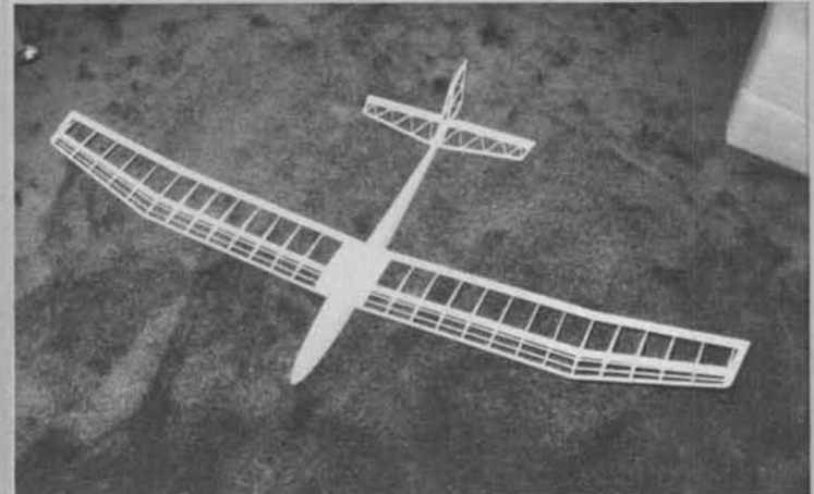
Test-fitting of all parts, and now ready for covering.
