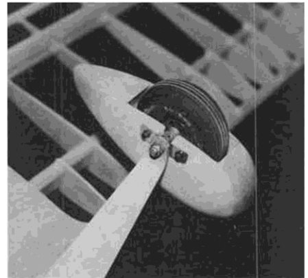
Wheel pants add a lot of class to any model. On this one, the pants are held in place by the same nut that secures the axle to the sheet aluminum landing gear.
