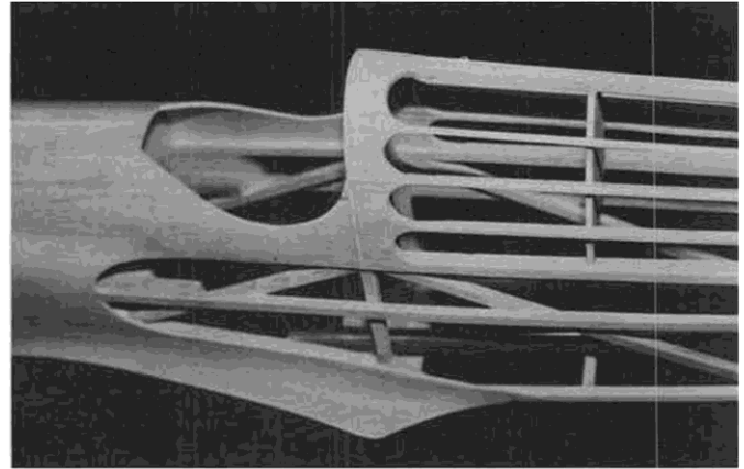
The cockpit area, showing the stringer fillets at former F-3A. Little details like this make a big difference in the finished job.
