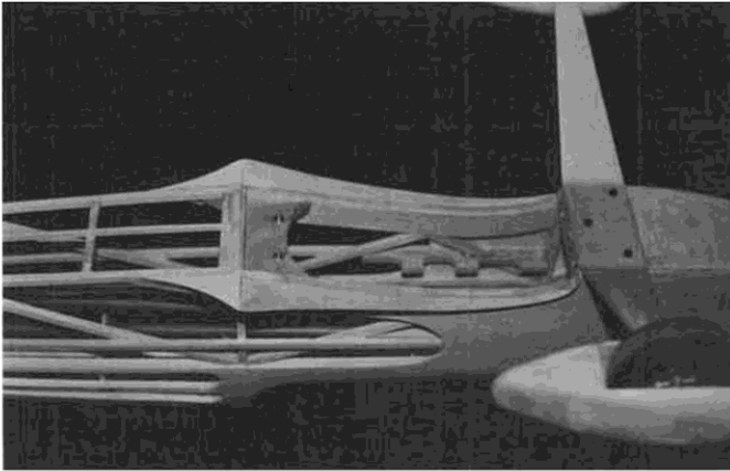
Landing gear and wing saddle detail. Note also the plywood wing attachment plate and servo tray.
