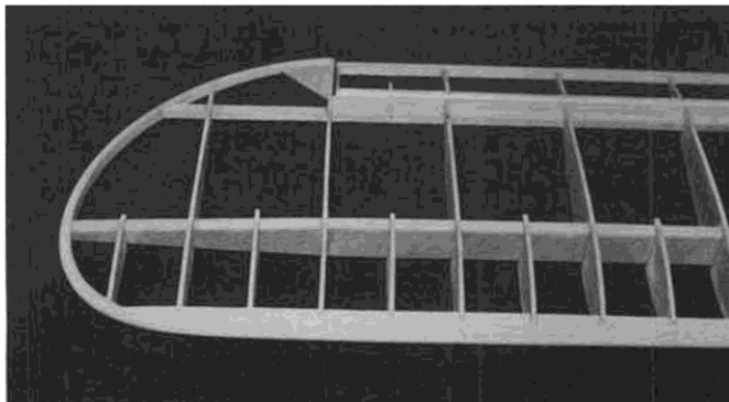
Wingtip with all structure sanded to final shape. Note how the leading edge is notched for the ribs. Spar web grain is santed 30° from vertical.
