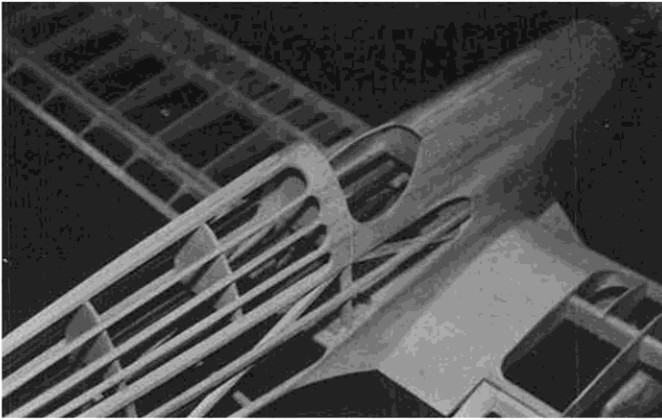
Wing fillets are Sig Epoxolite over a 1/32 ply base. Fillets are applied after the front end of the fuselage is fiberglassed.
