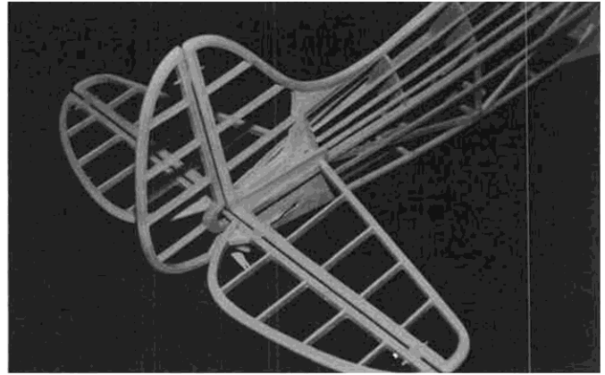
Tail surface outlines are laminated from basswood strips for a more realistic appearance. Simple technique is fully explained in text.
