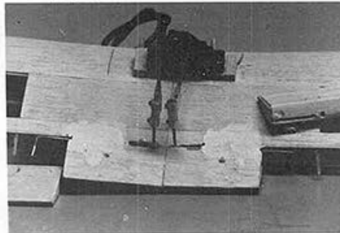
Aileron servo installed in wing.
