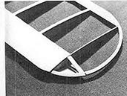
Closeup of wing tip detail, showing cap strips on ribs, leading edge sheeting.
