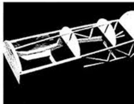
Forward fuselage construction detail.
