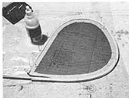
Detail of lamination of rudder outline. The technique is similar to that of the wing tips.
