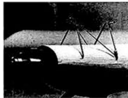
O.S. 10FSR installed. Note upper wing mount using blind nuts; clean and easy attachment.
