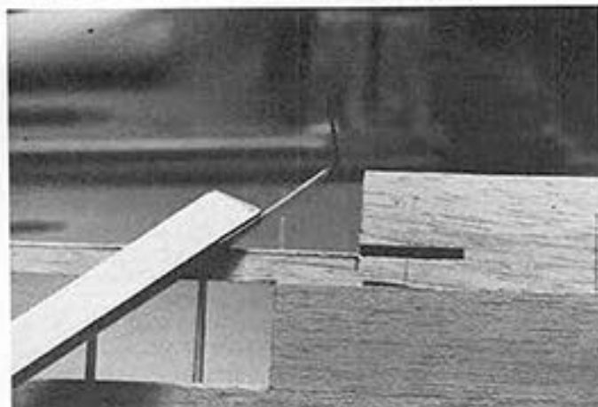
Detail shot of aileron structure and installation in wing.
