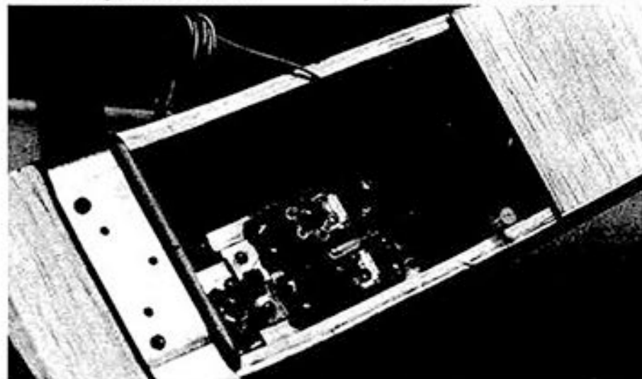
Alternate radio installation layout, using Cox/Sanwa four-channel with micro servos.
