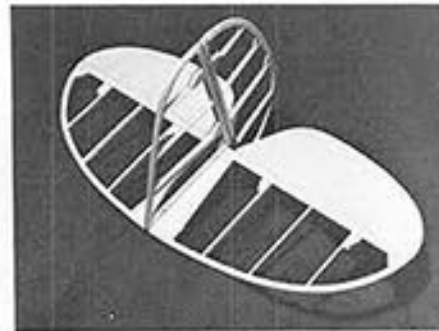
The completed rudder and elevator, ready for covering. Laminated surfaces are neat.
