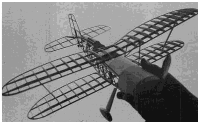
The author with his attractive biplane. Large stab area is evident in this photo.
