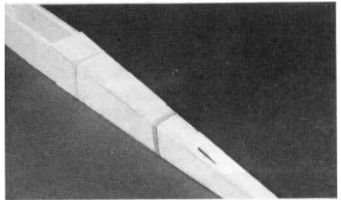
D 8. Trial fit the 3/32" Balsa Rear Top Fuselage Sheet (SPRTF04) in place*, and when satisfied with its fit apply a bead of thick CA along the 1/8" balsa stringers, the fuselage doublers and the fuselage sides and glue it in place. *NOTE: The top sheeting should be installed so the rudder pushrod cut-out is on the left side of the fuse. Check the plans for the proper orientation.
