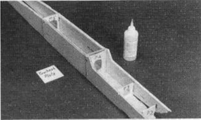
fuselage bottom with thick CA. Use the fuselage sides to help position it.
