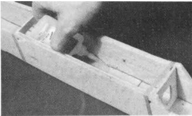
D 5. Spread the fuselage sides out and apply thick CA to formers F4 and F5 and the fuselage bottom between them. Reassemble, check to make sure the sides are pressed firmly against the formers and the bottom is fully seated against the sides, and allow the glue to cure.
