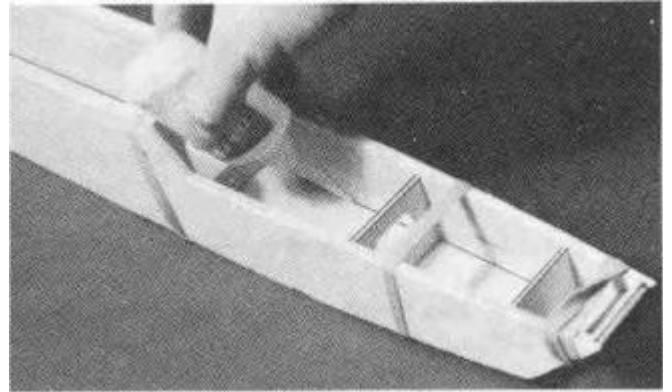
D 7. Pull the front fuselage sides together and trial fit the 1/8" Plywood Former F1 in place. Apply thick CA to the front fuselage bottom and the formers, install F1 and pull the fuselage sides together. A few rubber bands can be used to help hold the assembly while the glue cures.
