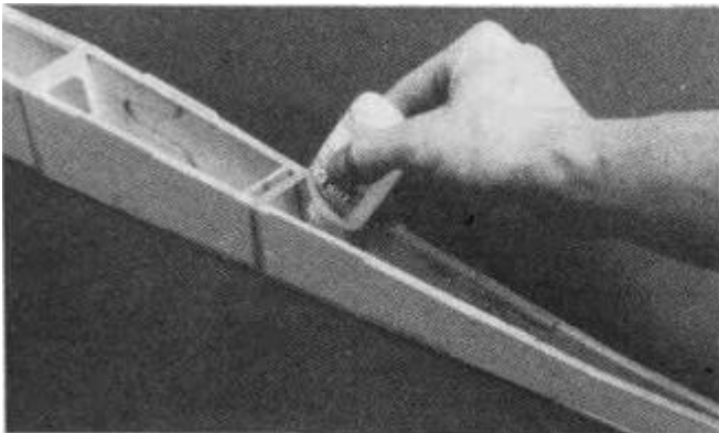
D 6. Pull the rear fuselage sides together and make sure that the sides are pressed firmly against former F6 and that the bottom is fully seated against the fuse sides. A couple of C2 clamps can be used to hold the tail of the fuselage together and rubber bands will help around the formers. Apply a couple of drops of thick CA on the back edge of the rear fuselage doubler and a bead of thin CA along the bottom sheeting
