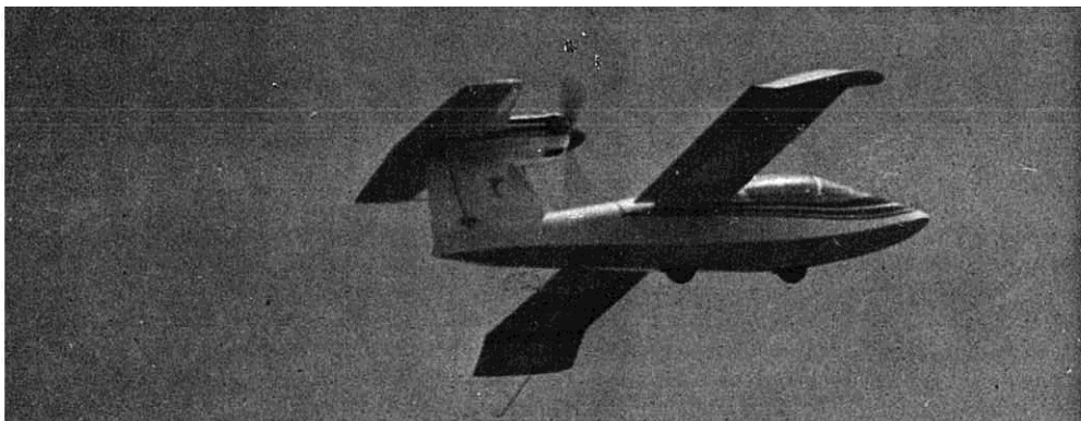
One of Spectra prototypes flies with S.T. .60, Heath radio on rudder, elevator, ailerons, flaps and throttle.
