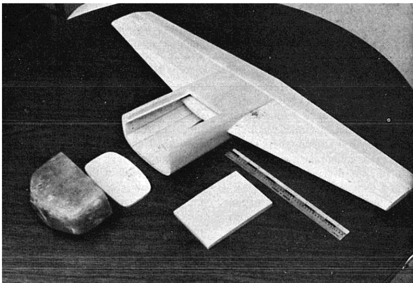
ABOVE: Fuselage planked on one side. BELOW: Engine nacelle and horizontal stabilizer assembly.
