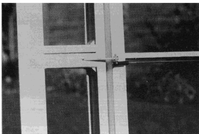
Aileron horn and linkage.
