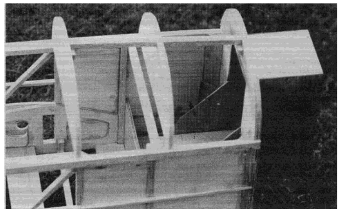
Looking inside fuel tank compartment. Note hook on far side for rubber band to secure tank.
