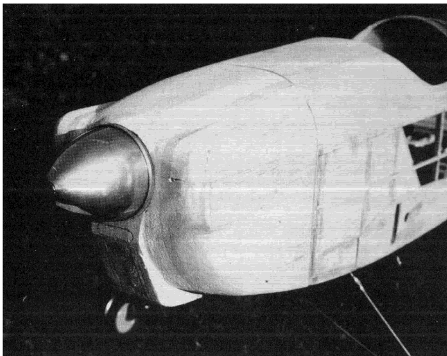
Balsa block cowling rough shaped. A fiberglass one including cylinders molded-in is available from T & D Fiberglass Specialties. See plan ad.
