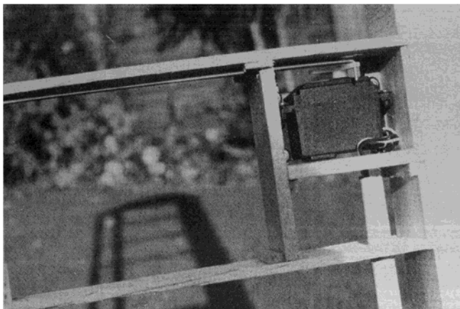
Servo mounted in each wing panel. Straight rod to aileron. Paper tube for servo wiring to travel to receiver.
