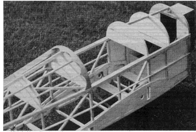
Close-up of cockpit area.
