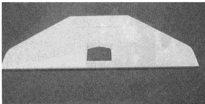
Wing inverted. Note landing gear block and cheater hole.
