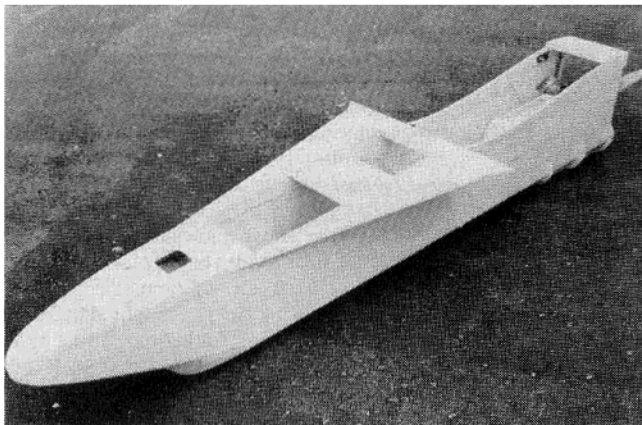
L.E.X. glued in place. Note the opening for the tuned pipe in front of air inlet hole.
