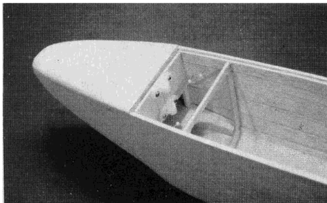
Nose gear mounting hardware is attached to plywood former and glued in place.
