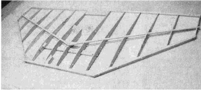
Wing is assembled in one piece on a flat building board. Note gussets at L.E.
