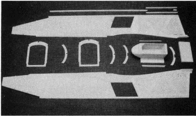
Fuselage sides, formers, fuel tank box, and balsa strips, ready for assembly.
