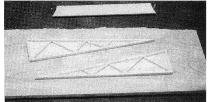
L.E.X. (leading edge extension) assembled in three pieces.
