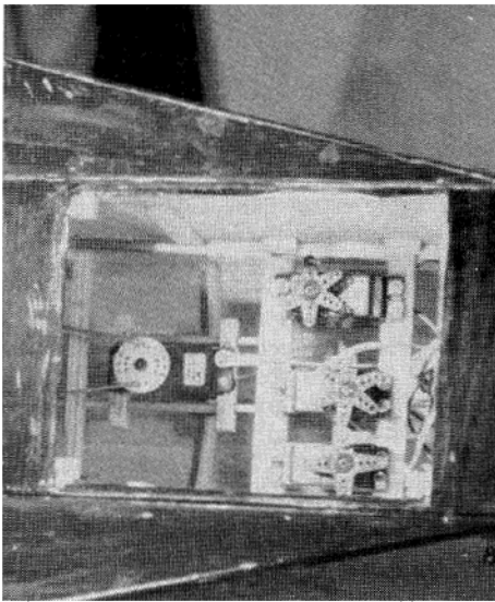
Servo installation. Note sliding tray set-up for elevons.
