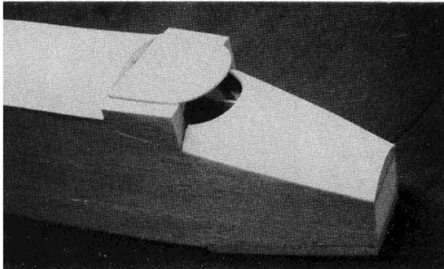
Nose section with canopy side blocks and top nose sheeting in place.
