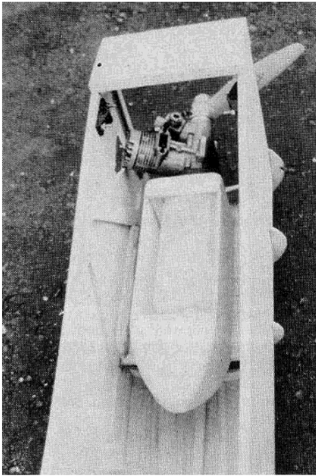
Rear wing bolt mounts installed and fuel tank box/engine mount glued in place.
