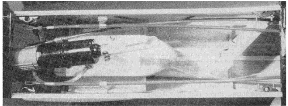
Elevon and throttle linkage. Be sure to anchor outer housings to fuselage sides to prevent flexing. Note exhaust tube with slit in end.
