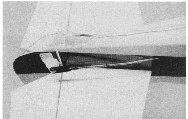
Pushrods and control horns. Loop the antenna through two holes drilled in the Goldberg wing skid used for a tail skid.
