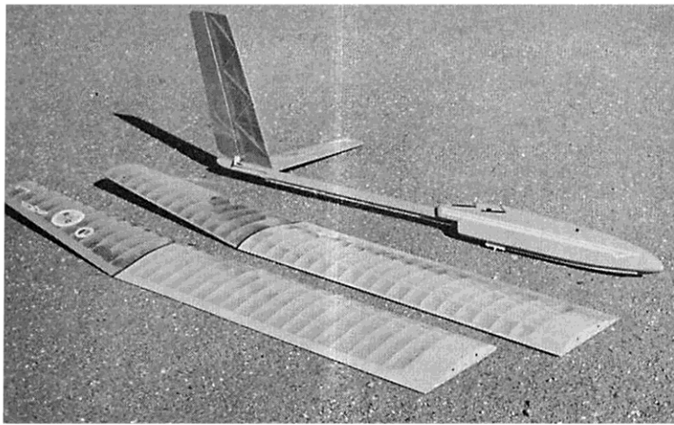
Translucent gleam of the ironed-on film gives you an idea of the structure. A thin fuselage, equipment in tandem arrangement. Light, thermals in winter air. At right: Temperature 22 degrees, thermals all over. It flies superbly.
