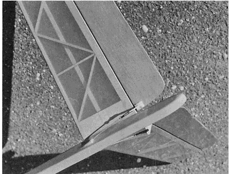
The "V" tail, easily built, nice in that it is graceful, high above ground on the landing roll. Popular on full scale soarers for this reason. Linkage can be seen on photo to right. Two horns are required. Bottom right photo captures the winch mechanism, foot treadle etc. Or use a hi-start line deal. Beneath: The nose, no room lost for a thin cross-section. It balances well.
