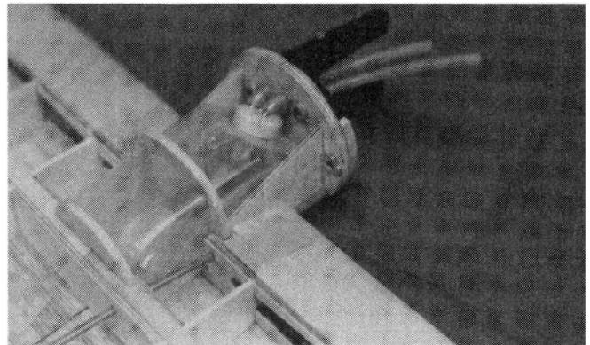
Nacelle formers, wing leading edge sheeting filled in, and throttle cable installed.
