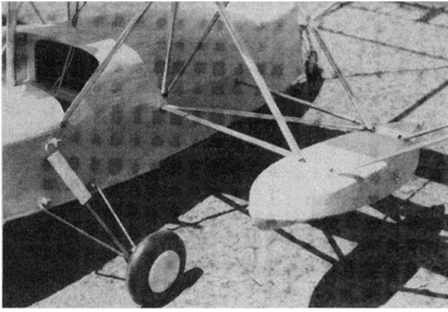
Wing mount and float strut detail.
