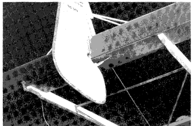
Rudder control detail.
