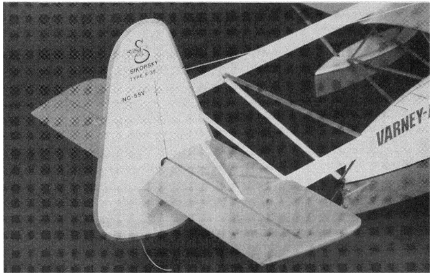
Tail detail. Note fin braces, 1/8" x 1/4" spruce.
