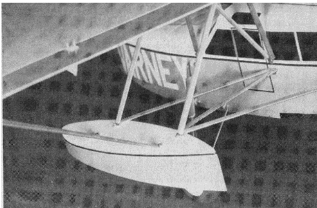
Float mount and wing strut detail.
