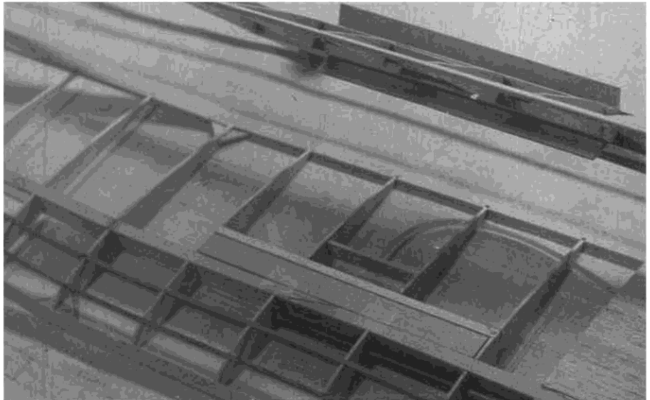
Spoiler details. Rear view of wing at top of photo shows top and bottom spoilers open. Also, note the optional ballast tubes just in front of the main spar. Lots of options on this model!
