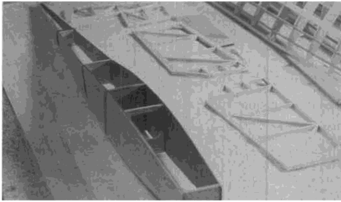
Fuselage structure without top and bottom sheathing. With full-length 1/64 ply side doublers, that fuselage should never break!
