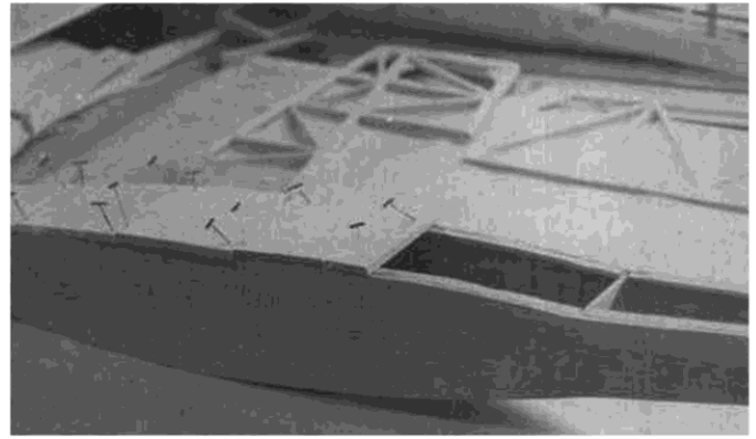
Use of thick top and bottom sheathing and triangular stock in corners permits well-rounded edges on finished model.
