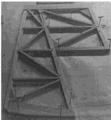
Both the rudder and stab can be completely assembled before taking them up off the board. Rudder is designed not to break if the ship flips over in an overzealous attempt to hit the spot. Extensive use of notching provides extra strength.
