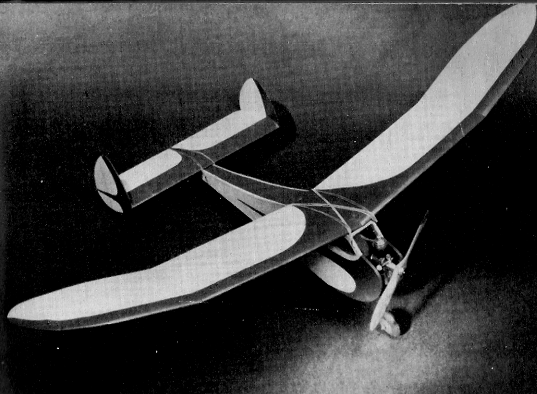
Sheet balsa nose sides, rubber band wing anchors and celluloid covered cabin are clearly defined in this photo of our Classy Gassy II. Note how twin rudders hold model upright despite single wheel landing gear.
