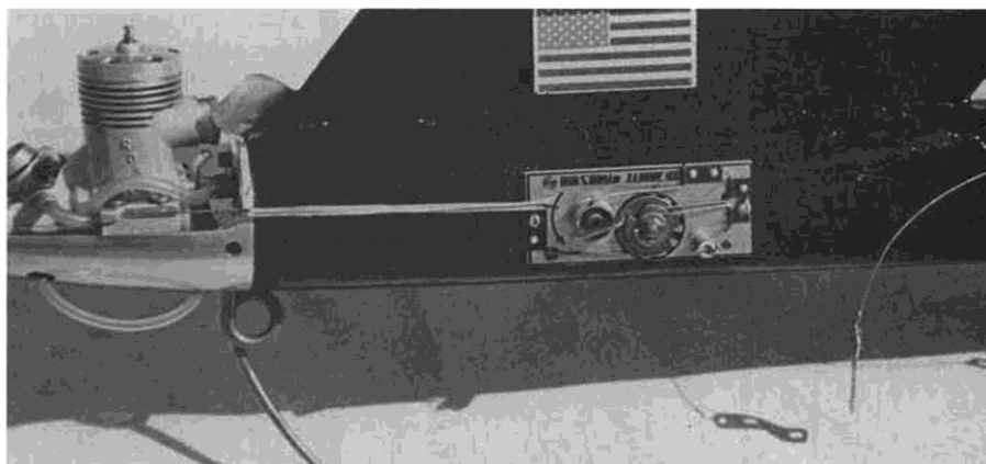
Timer rigging for flood-off system. Timer releases pinched pressure line from tank, dumping fuel into carb . . . blurp!
