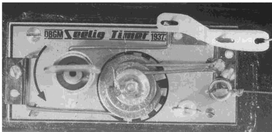
The single line V.I.T. fitting in climb position. First release puts stab in glide trim, second release is DT. Line with ring is to auto-rudder.
