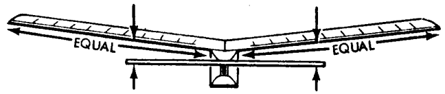
LEVEL STAB WITH RESPECT TO WING
